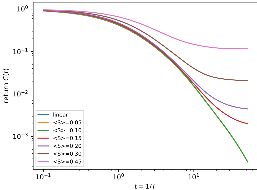
BI relaxation return ( q=17 )
