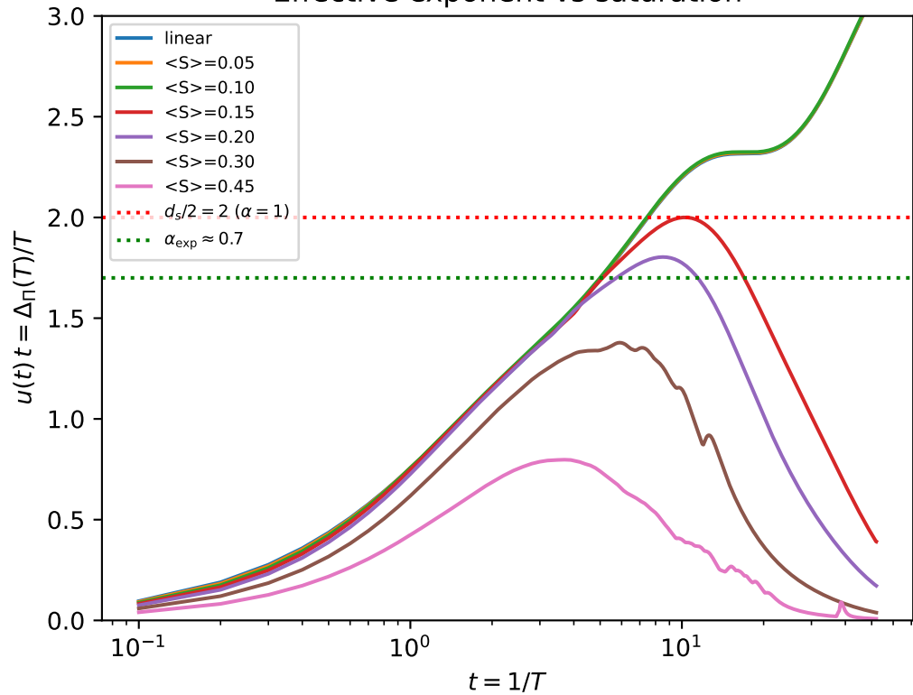
Effective exponent vs saturation
