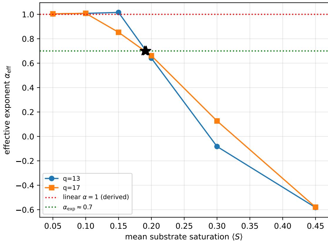
BI bends \alpha : 1 \rightarrow 0.7 at \langle S \rangle \approx 0.19 (window t \in [6, 12] )
