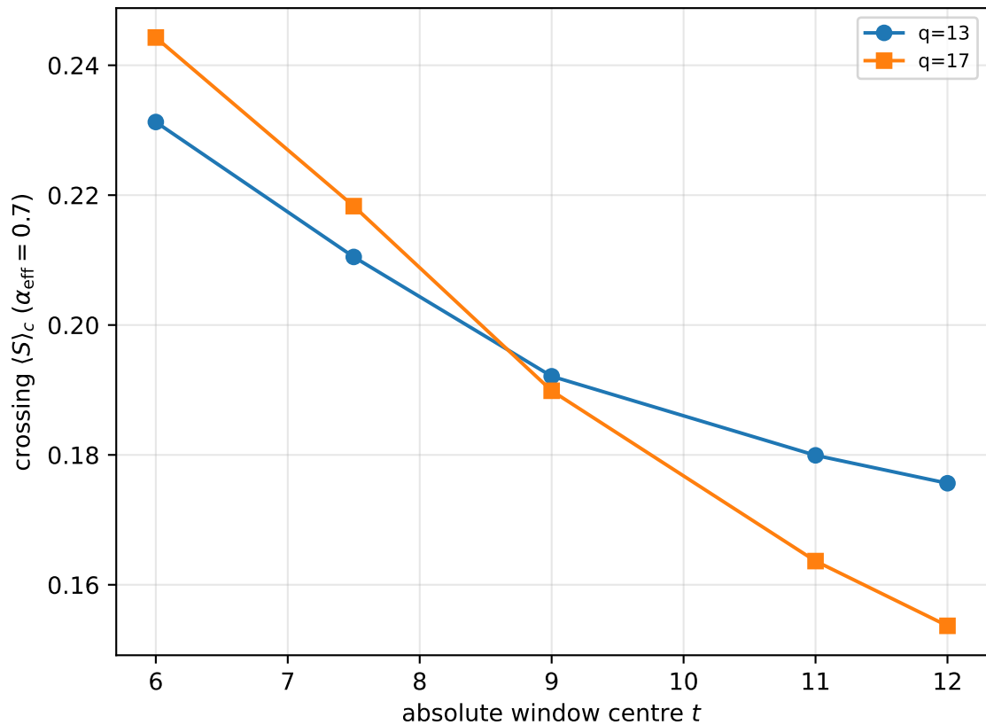
q-stability and running of the exponent
