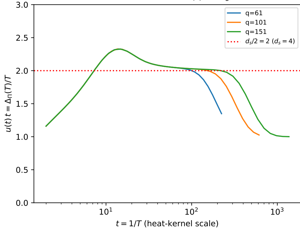
Planckian closure: u(t) t \rightarrow d_s/2
