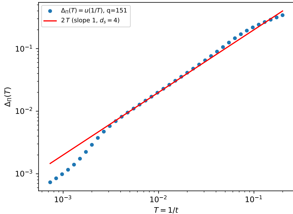
Linear thermal closure \Delta_{\Pi}(T) \sim 2T
