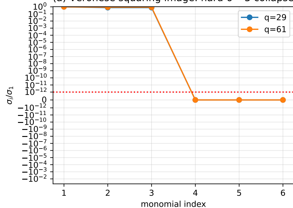
(a) Veronese squaring image: hard 6 \rightarrow 3 collapse
