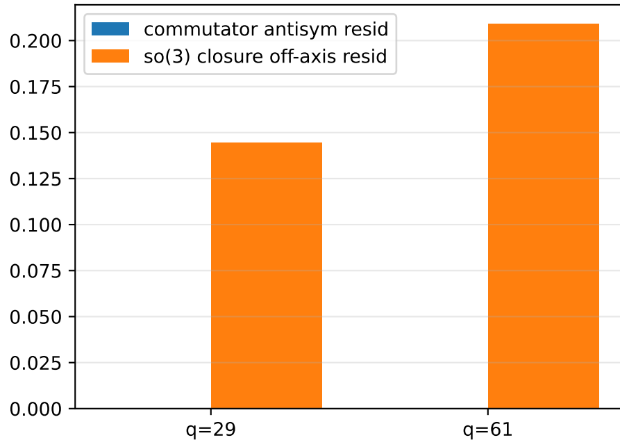
(b) constraint forms: \mathfrak{so}(3) -valued but not exactly closing
