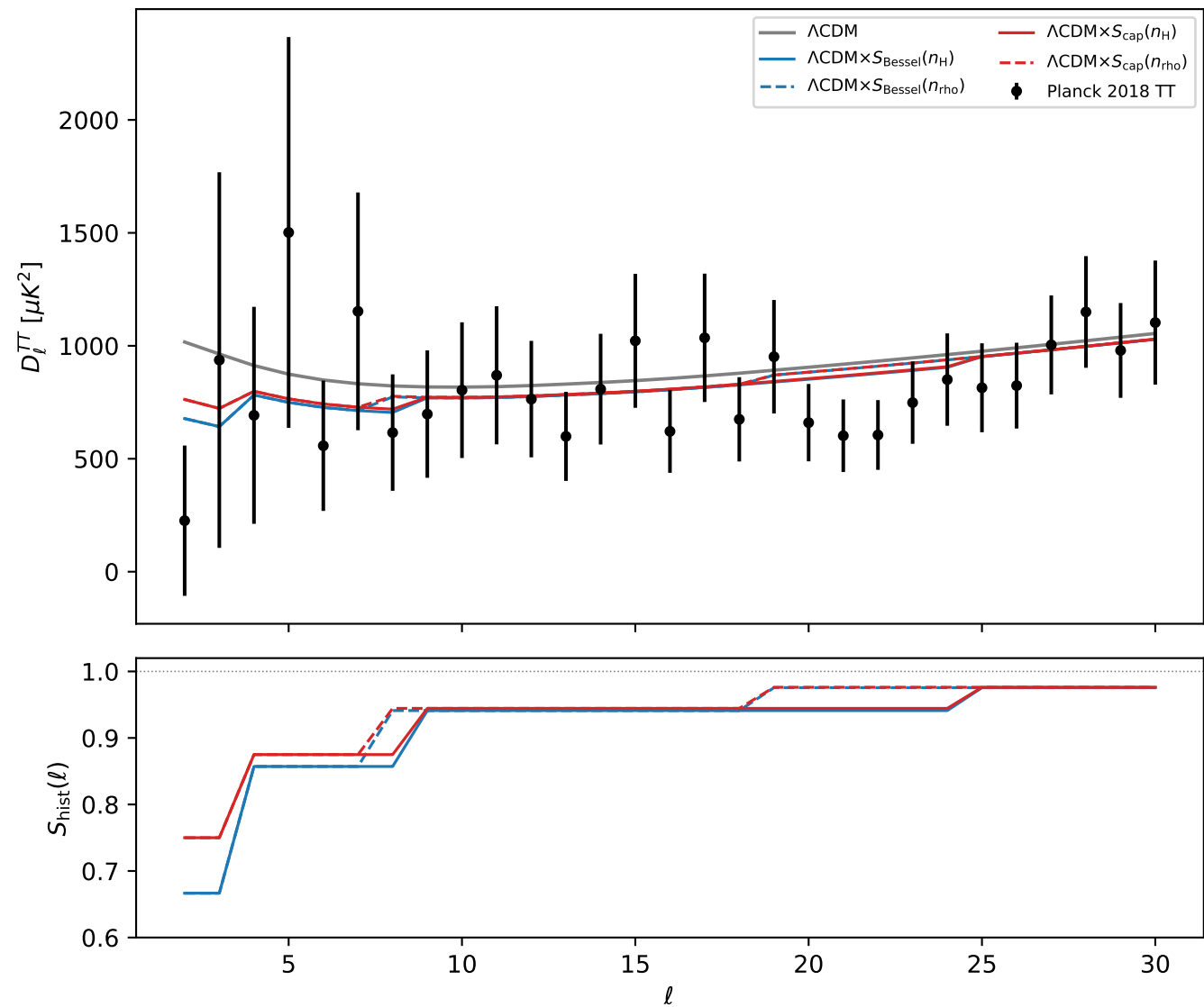
Distinguishable-history capacity envelopes vs Planck TT (no fit, quadrupole-anchored)
