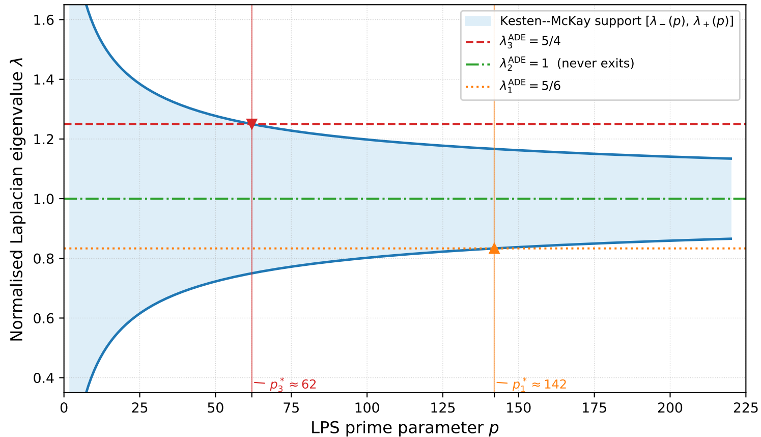
Kesten-McKay support contraction and ADE level exit order ( 2I , ord-5, |S| = 24 )
