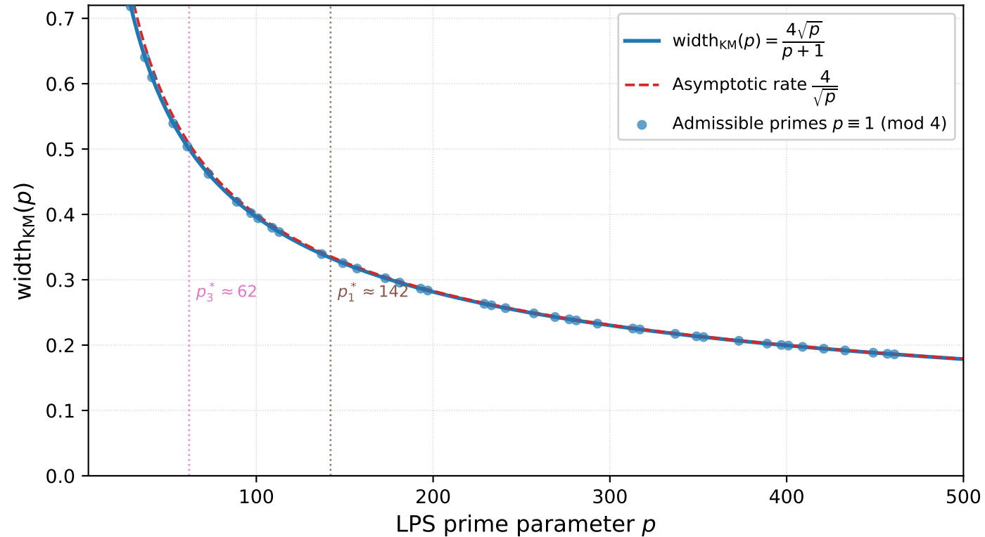
Kesten--McKay window width and asymptotic rate (Proposition~1)
