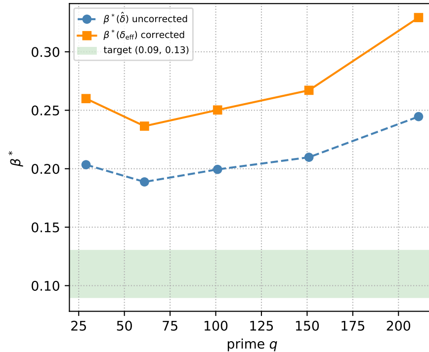
(B) \beta^* : uncorrected vs corrected
