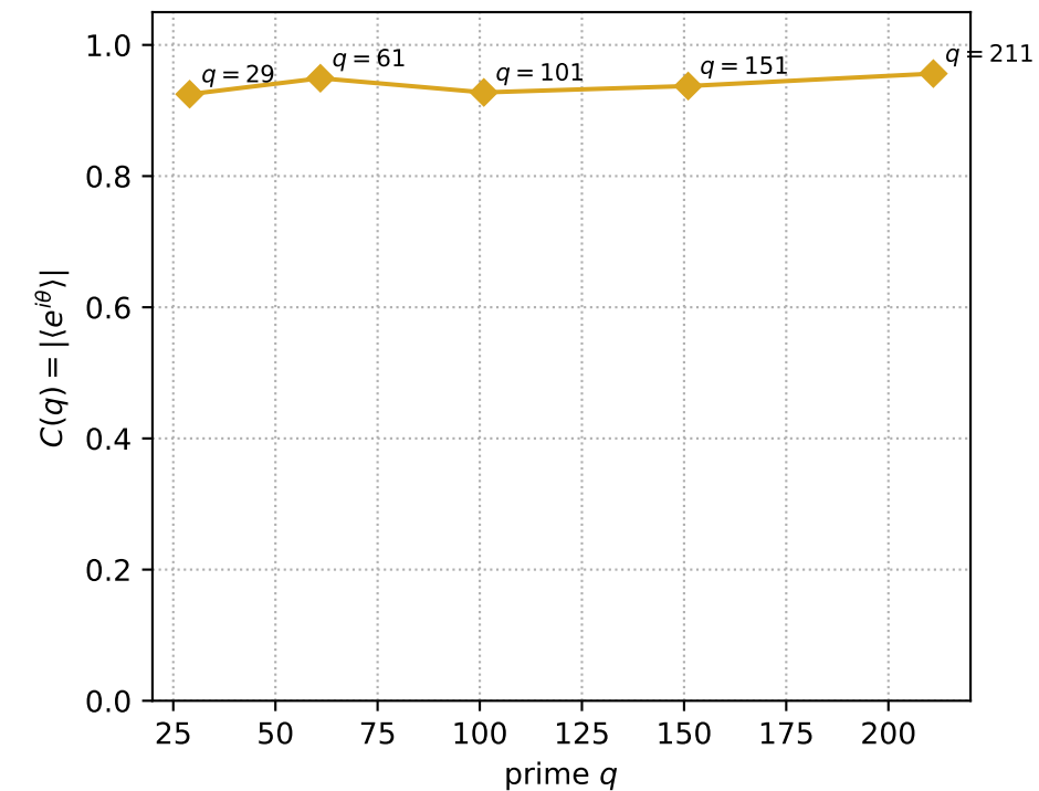
(F) Phase coherence factor C(q)
