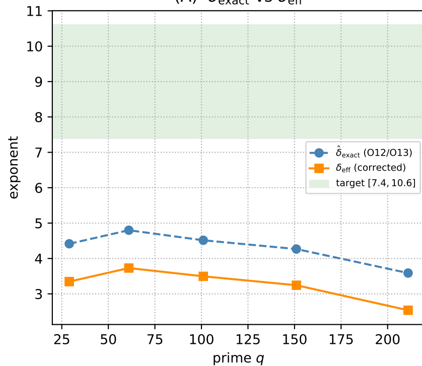
(A) \hat{\delta}_{\text{exact}} vs \delta_{\text{eff}}
