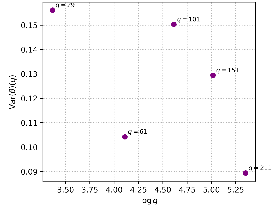
(C) Circular phase variance vs \log q
