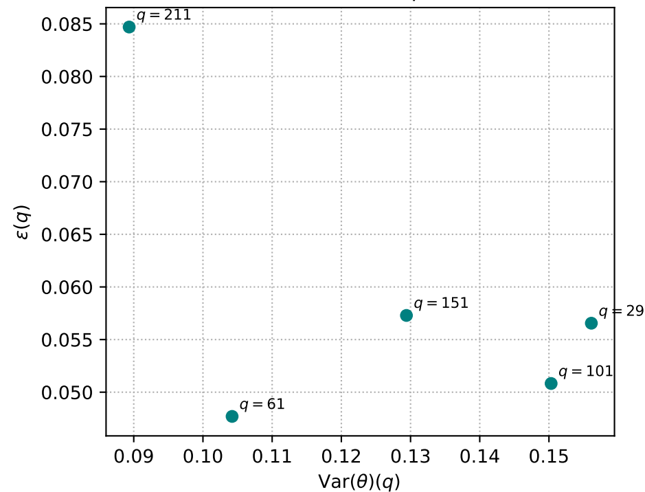
(E) \varepsilon(q) vs \text{Var}(\theta) — key result Pearson r = -0.575 , p = 0.3109
