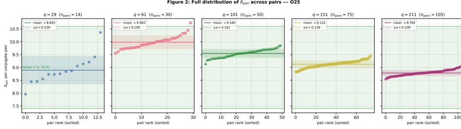
Figure 2: Full distribution of \delta_{\text{pair}} across all conjugate pairs for each prime, sorted by value. Horizontal line: mean \bar{\delta}_{\text{pair}} . Shaded band: \pm\sigma_q . Green dashed lines: admissible window [7.4, 10.6] . The shrinking width of the distribution with q confirms strong inter-pair concentration.
