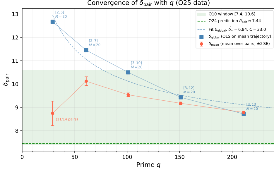
Figure 4: Convergence of \delta_{\text{pair}} with q from the extended O25 campaign ( q \in \{29, 61, 101, 151, 211\} , M = 20 , windows from the WINDOW_O12 table). Squares (blue): \delta_{\text{global}} , the OLS exponent on the mean \sigma_{\text{pair}} trajectory. Circles (red): \bar{\delta}_{\text{pair}} , mean over conjugate pairs, with \pm 2 SE error bars. Dashed blue: fit \delta_{\text{global}} \approx 6.84 + 33.0/\sqrt{q} , extrapolating to \hat{\delta}_{\infty} = 6.84 (slightly below the O24 prediction of 7.44, consistent with the known negative bias of \delta_{\text{global}} relative to \bar{\delta}_{\text{pair}} ). Green band: admissible window [7.4, 10.6] from O10. Green dashed: O24 prediction \delta_{\text{pair}} \approx 7.44 . The annotation (11/14 pairs) at q = 29 flags incomplete pair coverage due to short fitting window.
