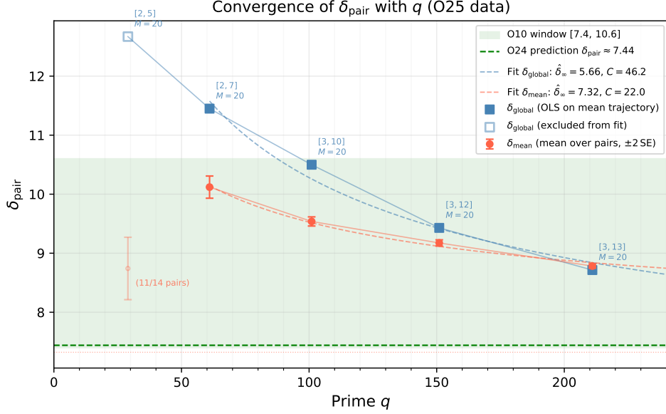
Figure 4: Convergence of \delta_{\text{pair}} with q from the extended O25 campaign ( q \in \{29, 61, 101, 151, 211\} , M = 20 , windows from the WINDOW_O12 table). Filled symbols: primes included in the extrapolation fits ( q \in \{61, 101, 151, 211\} ). Open/faded symbols: q = 29 , excluded from fits (only 11/14 pairs converge and the fitting window has 4 points; see §3.3 for the structural explanation). Squares (blue): \delta_{\text{global}} , the OLS exponent on the mean \sigma_{\text{pair}} trajectory. Circles (red): \bar{\delta}_{\text{pair}} , mean over conjugate pairs, with \pm 2 SE error bars. Dashed red: fit \bar{\delta}_{\text{pair}} \approx 7.32 + 22.0/\sqrt{q} , extrapolating to \hat{\delta}_{\infty} = 7.32 , within 0.12 of the O24 prediction of 7.44. Dashed blue: fit \delta_{\text{global}} \approx 5.66 + 46.2/\sqrt{q} , extrapolating to 5.66 (below O24, reflecting the known negative bias of \delta_{\text{global}} relative to \bar{\delta}_{\text{pair}} ). Green band: admissible window [7.4, 10.6] from O10. Green dashed: O24 prediction \delta_{\text{pair}} \approx 7.44 .
