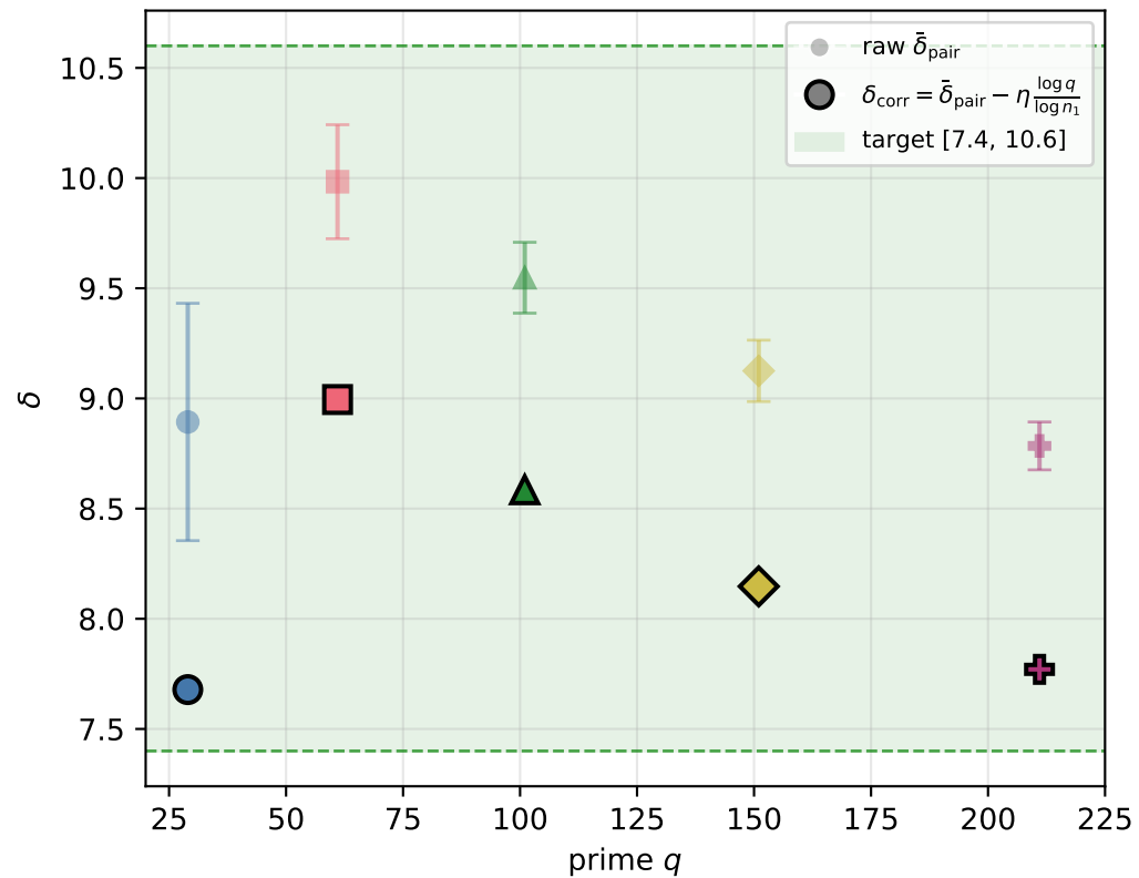
(B) Raw vs O14-corrected ( \eta = 1/2 )
