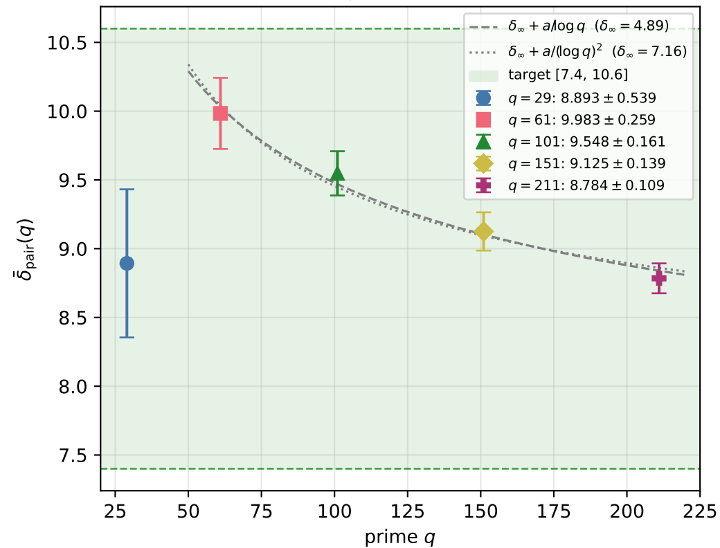
(A) Raw \bar{\delta}_{\text{pair}} and empirical fits
