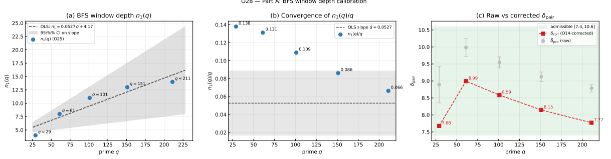
Figure 1: Part A: BFS window depth calibration over q \in \{29, 61, 101, 151, 211\} . (a) n_1(q) with OLS fit n_1 = \hat{a}q + \hat{\beta} and 95% confidence band. (b) Ratio n_1(q)/q : monotonically decreasing from 0.138 to 0.066, confirming Scenario S2 (pre-asymptotic regime throughout the tested range). (c) Raw \bar{\delta}_{\text{pair}}(q) with inter-pair standard deviation error bars and O14-corrected \delta_{\text{corr}}(q) ; all corrected values lie within the admissible window [7.4, 10.6] (shaded).
