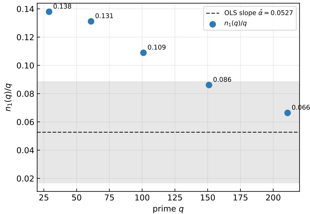
(b) Convergence of n_1(q)/q
