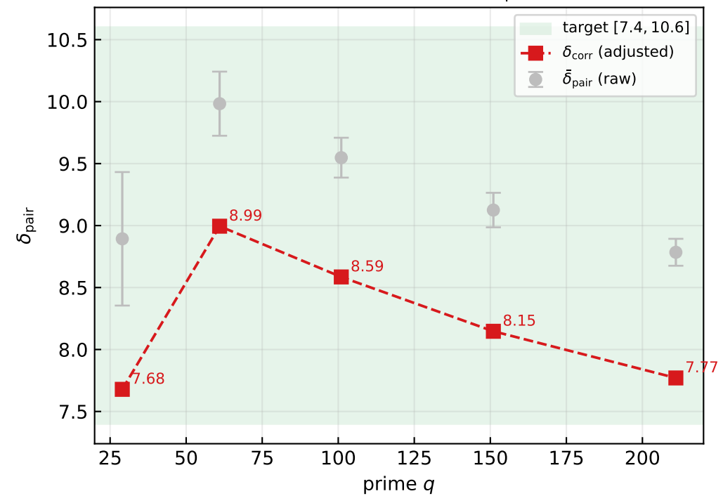
(c) Raw vs adjusted \delta_{\text{pair}}
