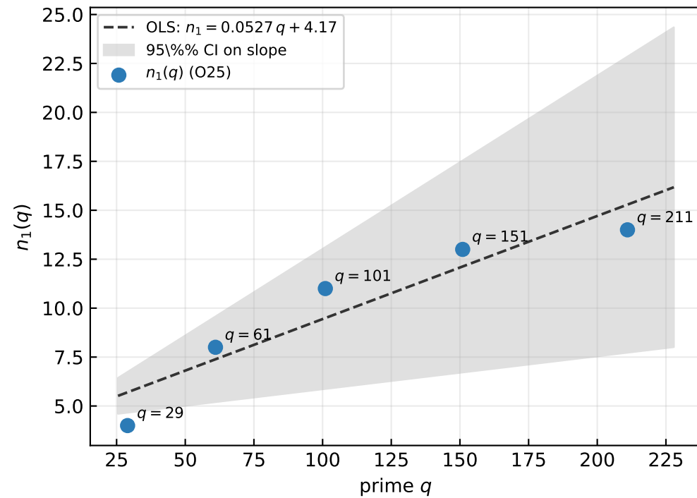
(a) BFS window depth n_1(q)
