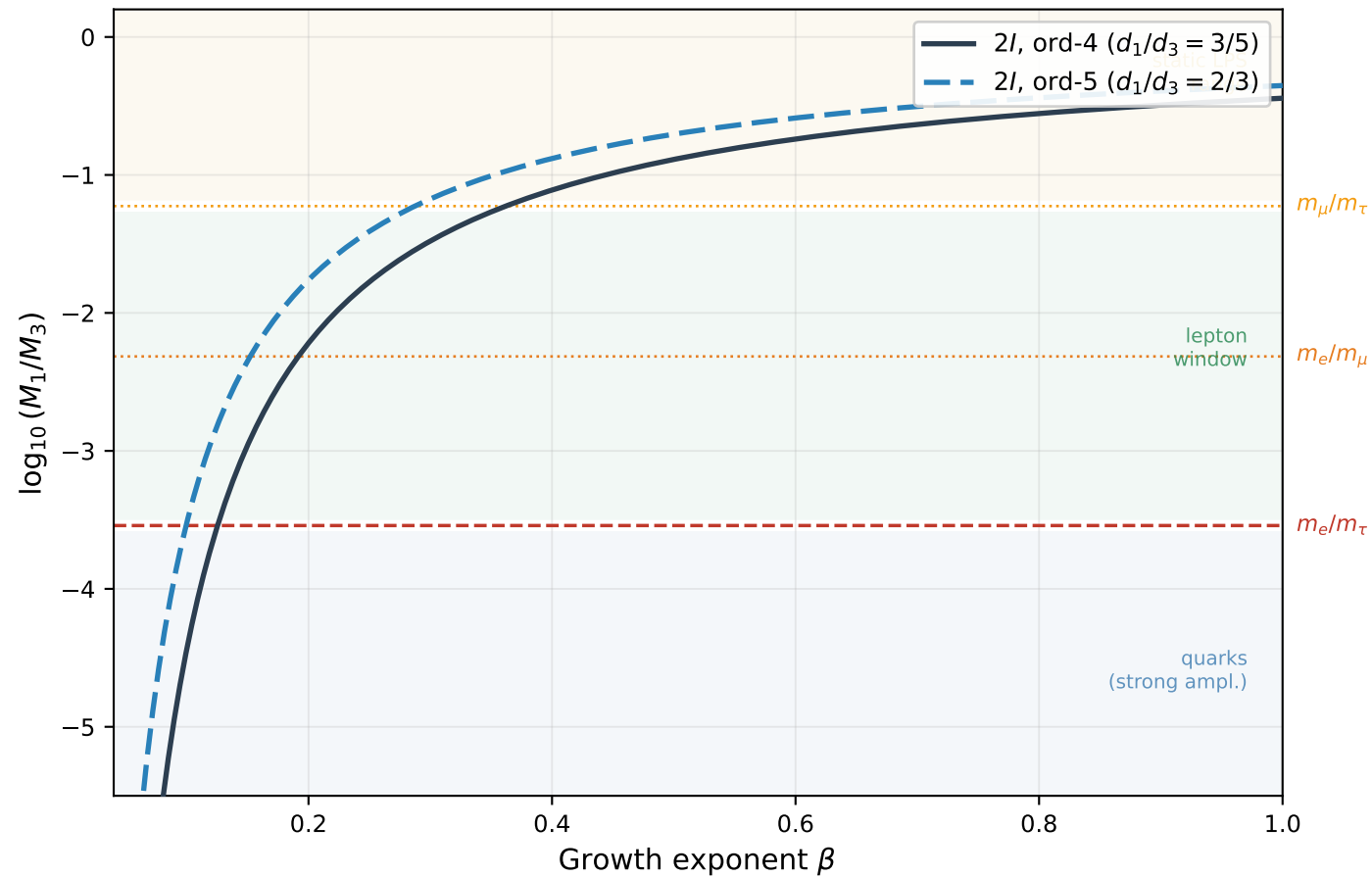
Mass ratio M_1/M_3 as a function of the growth exponent \beta
