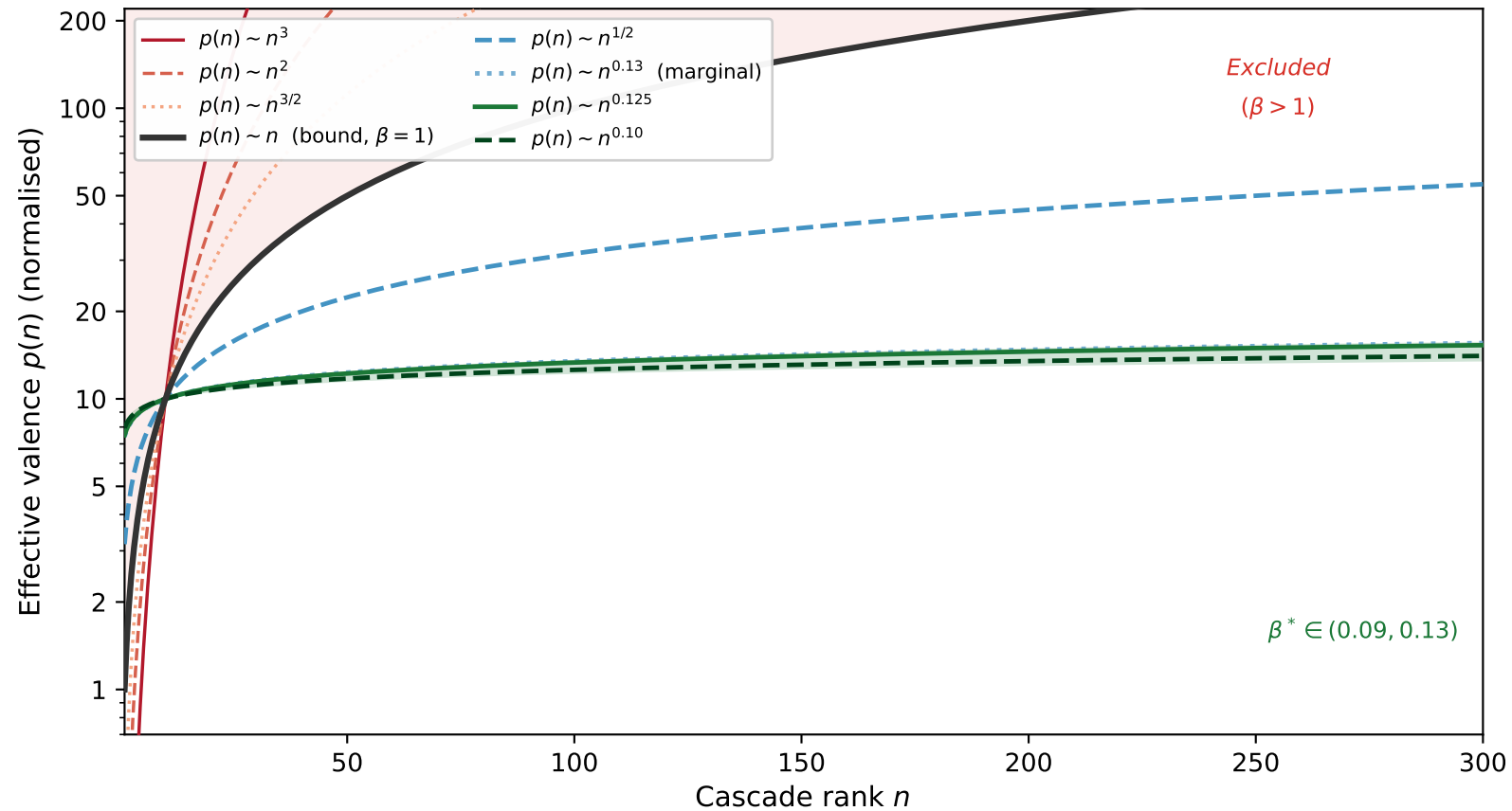
Valence growth laws: structural bound and phenomenological window
