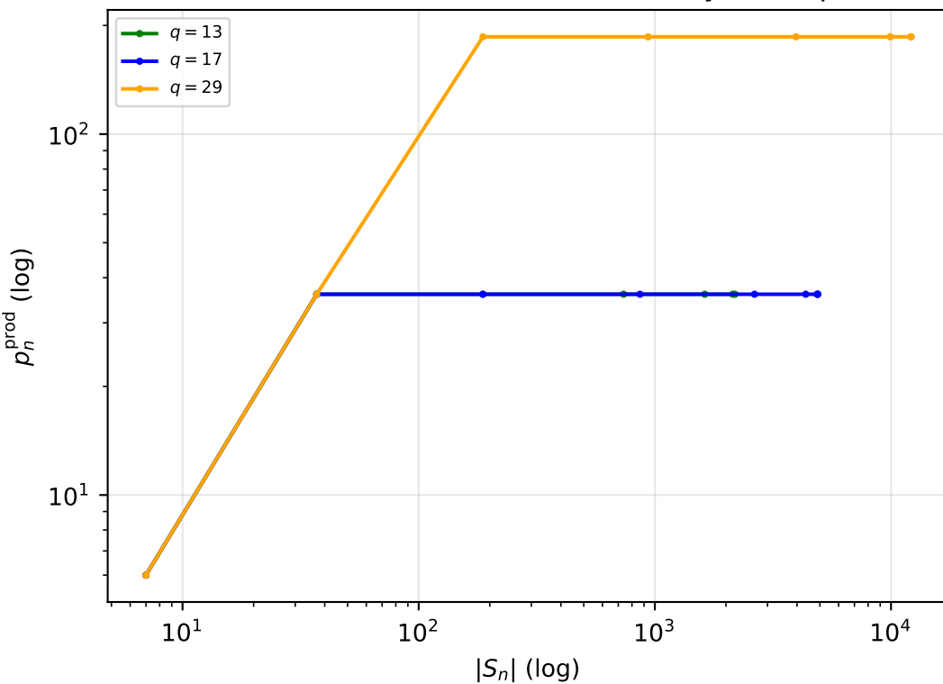
Cumulative admissible front (reference only; no exponent fit)
