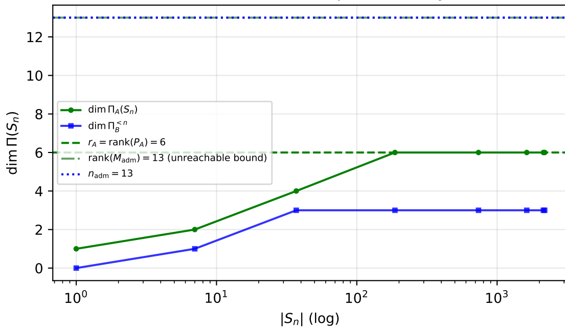
Finite bound r_n \leq r_A/|S_n| (Corollary~1)
