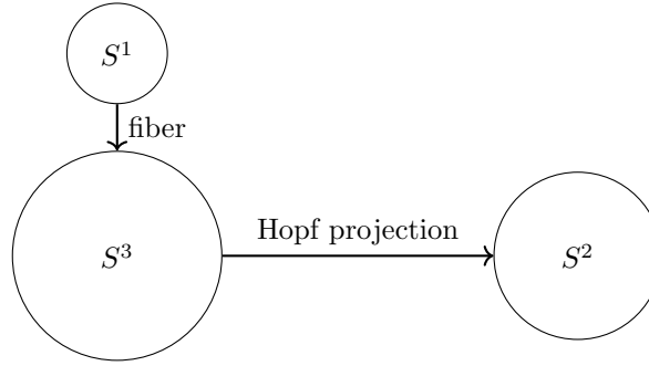
Fig. 2 Schematic representation of the Hopf fibration S^1 \hookrightarrow S^3 \rightarrow S^2 , illustrating the separation between fiber and base degrees of freedom.
