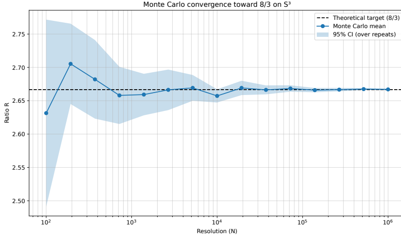
Fig. 3 Monte–Carlo convergence of the spectral ratio R = 8\langle \cos^2 \rangle / \langle \sin^2 \rangle toward the universal value 8/3 for uniform sampling on S^3 . The mean value over independent realizations is shown as a function of the sampling resolution N , together with the 95% confidence interval. The convergence illustrates the robustness of the ratio and its independence from discretization details.
