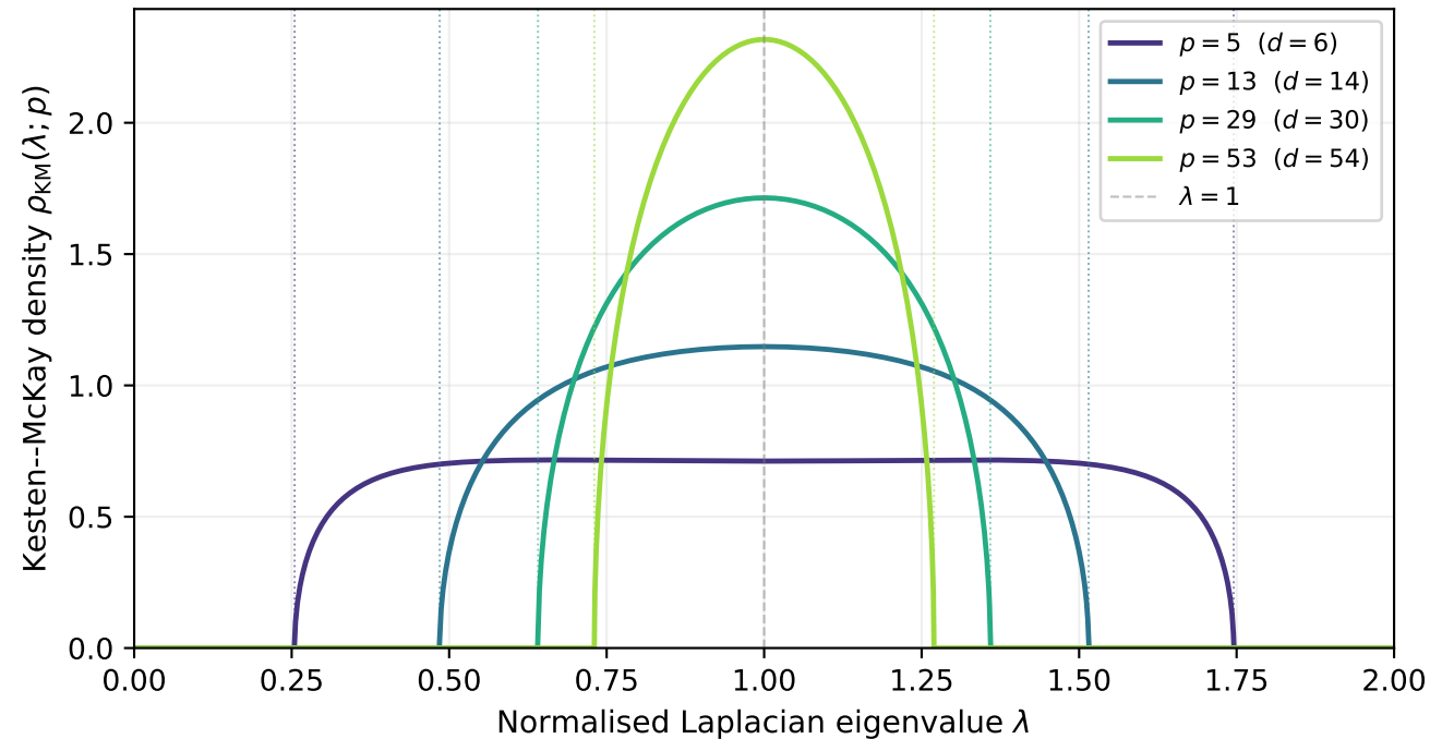
Kesten--McKay spectral density for various p
