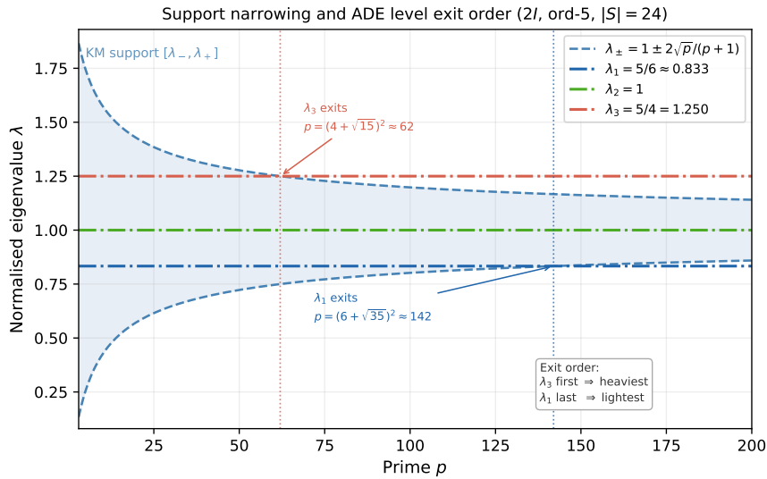
Figure 3: Kesten–McKay support edges \lambda_{\pm}(p) = 1 \pm 2\sqrt{p}/(p+1) as functions of the prime p , with the three ADE eigenvalue levels of 2I (ord-5, |S| = 24 ) shown as horizontal dash-dotted lines. As p grows, the support narrows : \lambda_+ - \lambda_- = 4\sqrt{p}/(p+1) \rightarrow 0 . The level \lambda_3 = 5/4 exits the support at p = (4 + \sqrt{15})^2 \approx 62 ; \lambda_2 = 1 never exits (it is the midpoint of the symmetric support); \lambda_1 = 5/6 exits at p = (6 + \sqrt{35})^2 \approx 142 .
