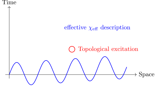
Fig. 1 Conceptual representation of Cosmochrony. An effective spacetime depiction of the projected scalar description of \chi , used for visualization purposes only. The monotone accumulation of projected spectral structure gives rise to an effective temporal ordering, while localized topological excitations correspond to particle-like configurations in the emergent geometric regime.
