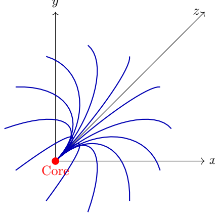
Fig. 17 Skyrion-like configuration of \chi_{\text{eff}} (spin- \frac{1}{2} ).
