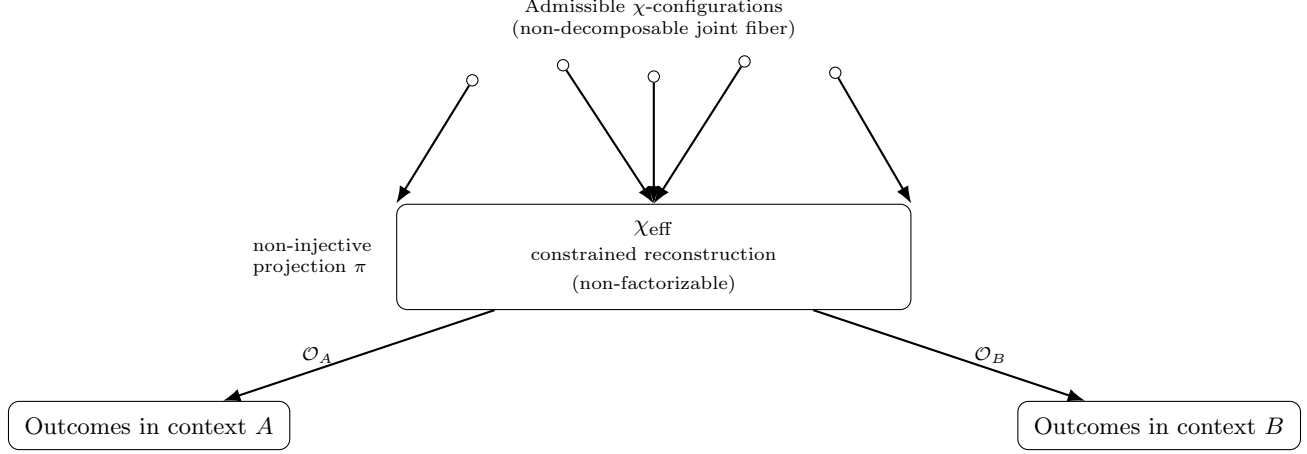
Fig. 10 Non-factorizable regime. The joint fiber \Pi^{-1}(o_{AB}) is non-decomposable: no independent pre-images can be assigned to subsystems A and B . The admissibility structure of \chi determines which balance invariants are infra-projectable; it does not select a unique pre-existing configuration. Different measurement contexts define distinct admissible reprojections of the same constrained fiber, producing correlated outcomes without superluminal influence.
