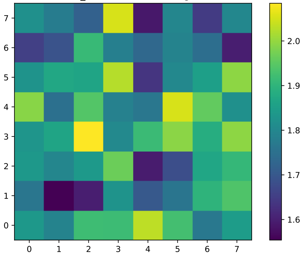
chi_eff slice (mid z) (rough)
