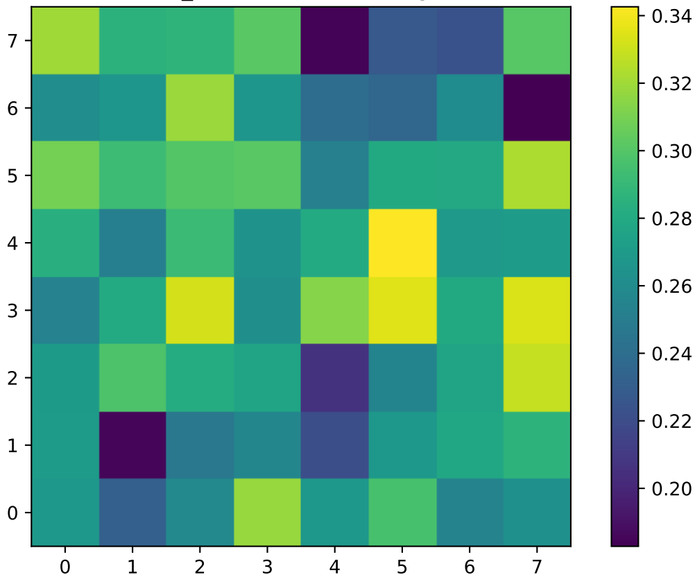
chi_eff slice (mid z) (rough)
