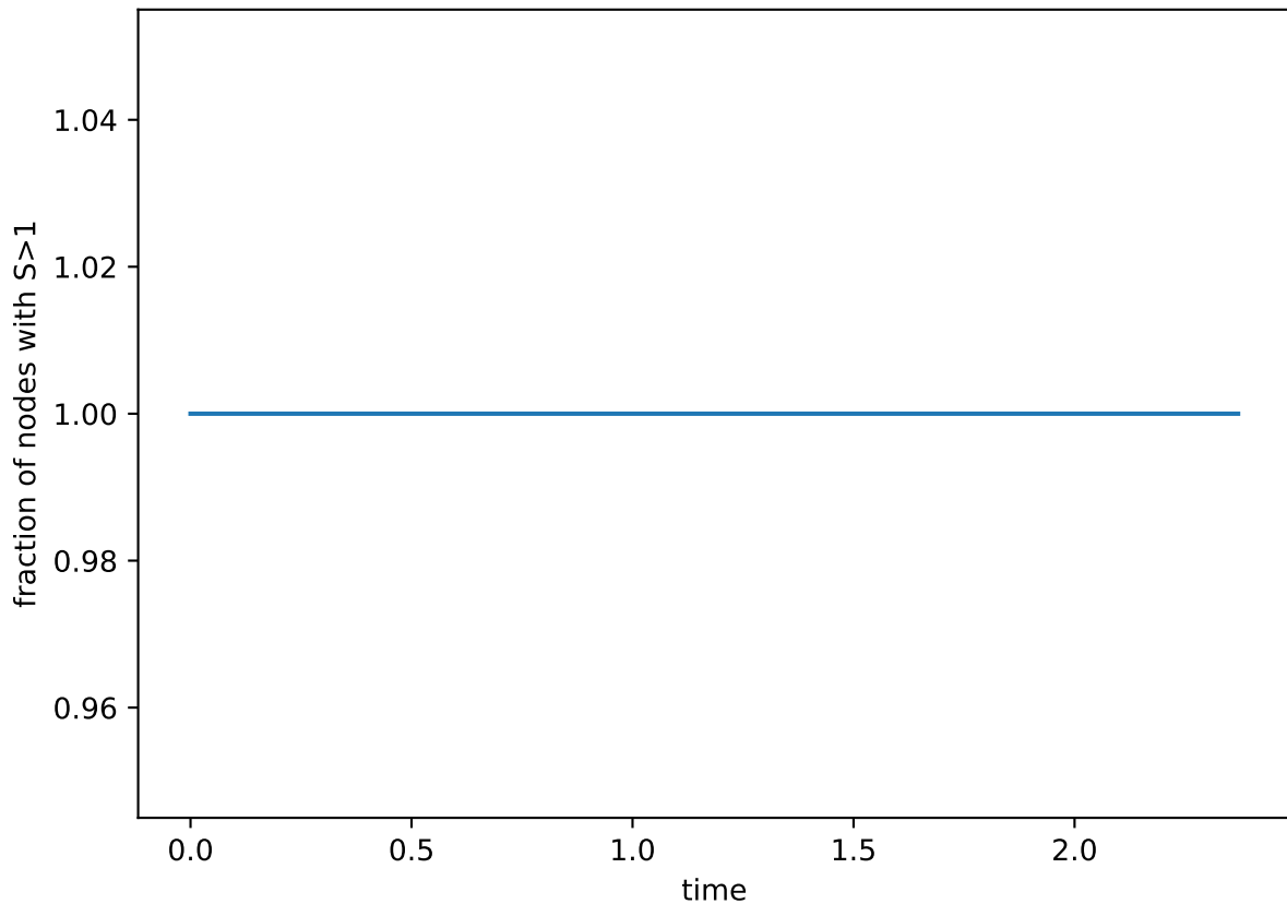
Saturation fraction vs time (nonprojectable)
