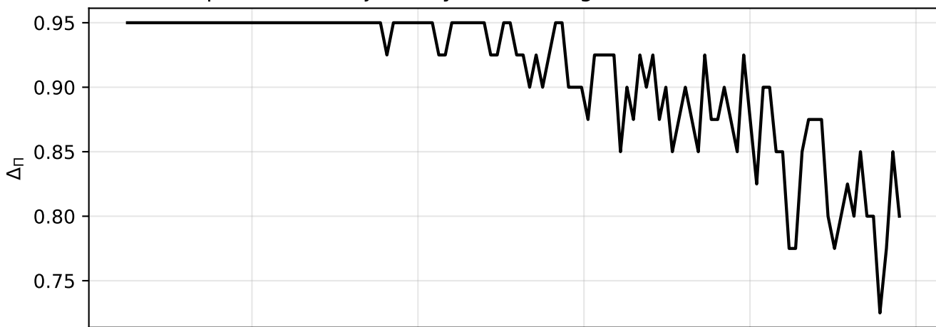
Spectral non-injectivity and entanglement intermittence
