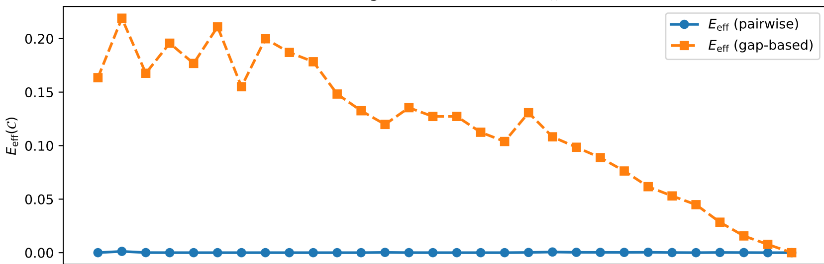
Effective entanglement observable: \Delta_{\Pi}(c)(1 - c^{\nu})
