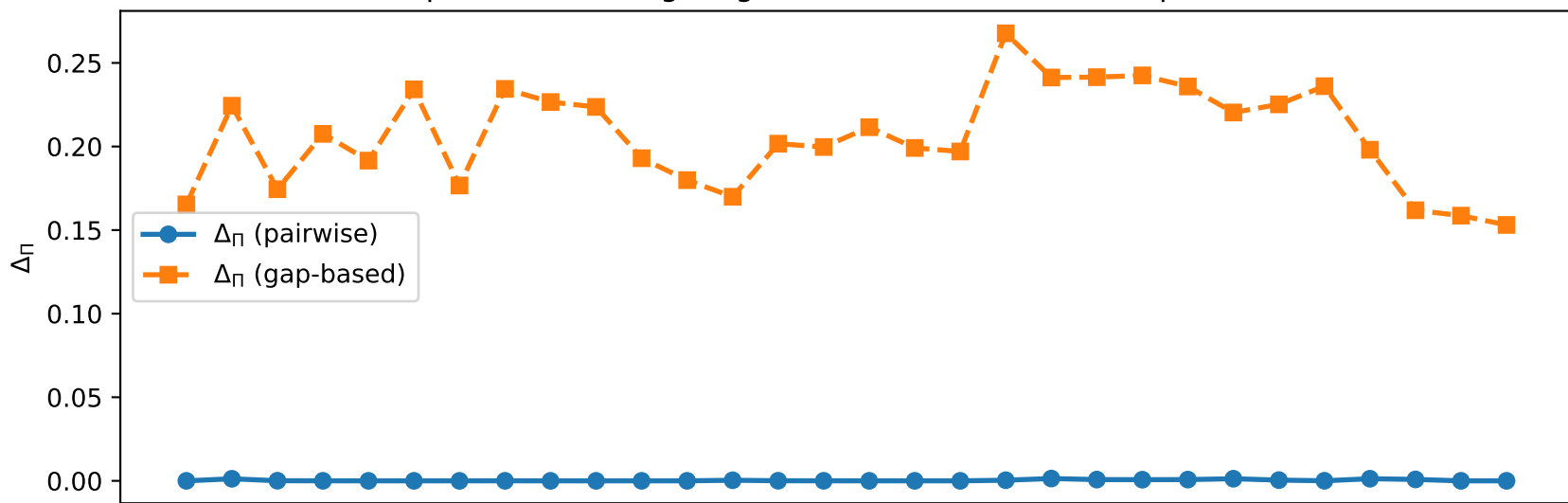
Spectral crowding diagnostics vs Born-Infeld compression
