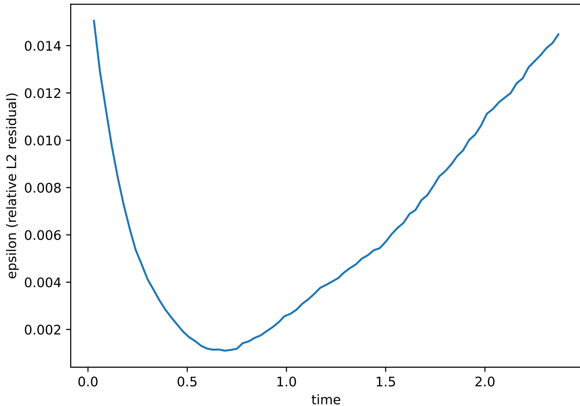
Epsilon vs time (rough)
