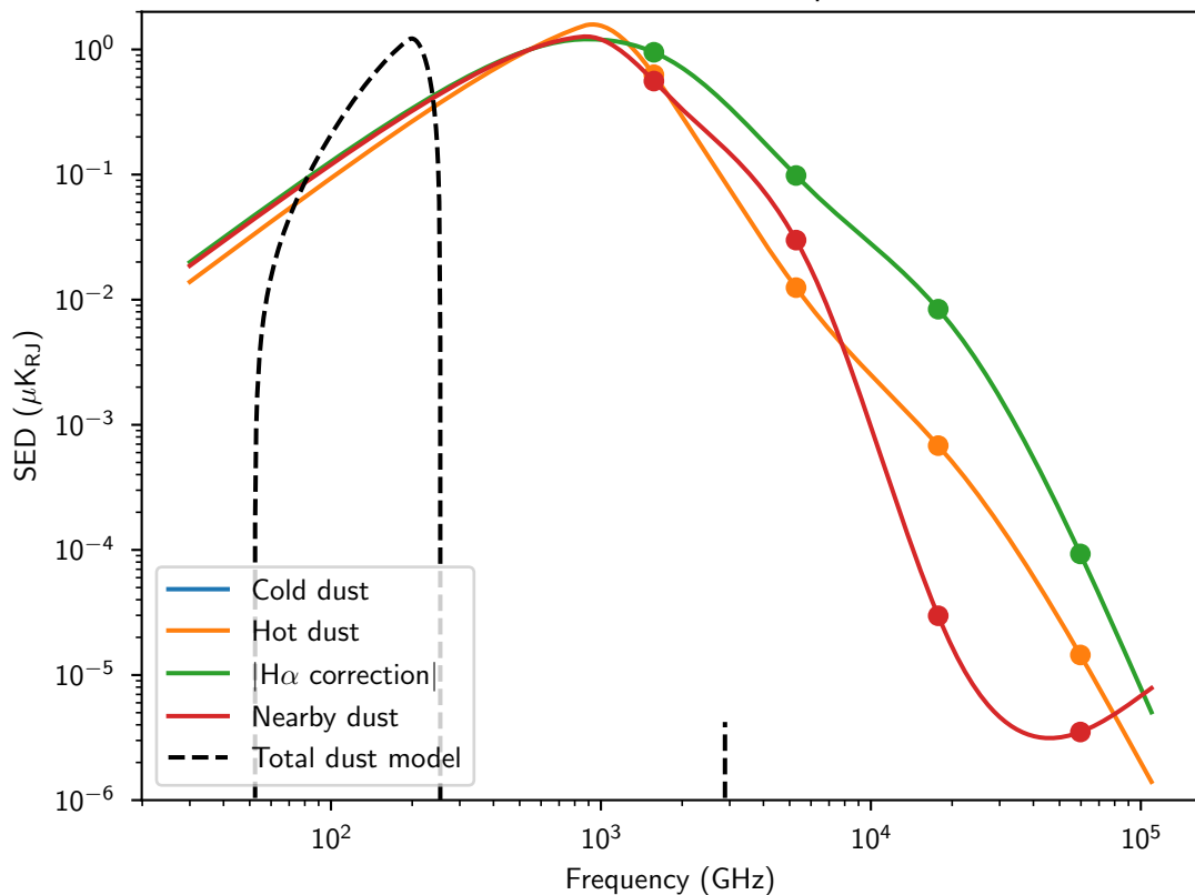
Final SEDs for all dust components
