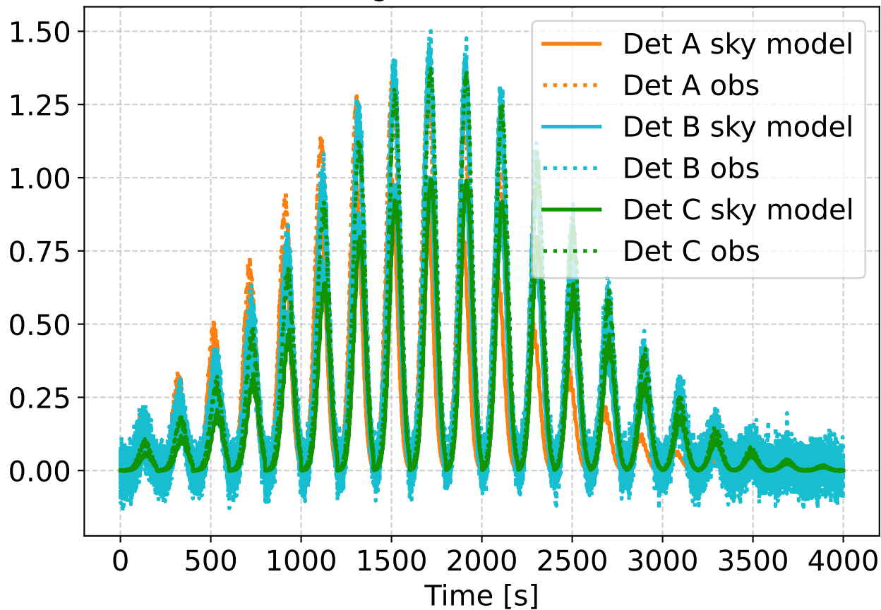
Simulated Signal with Cross-talk and WN
