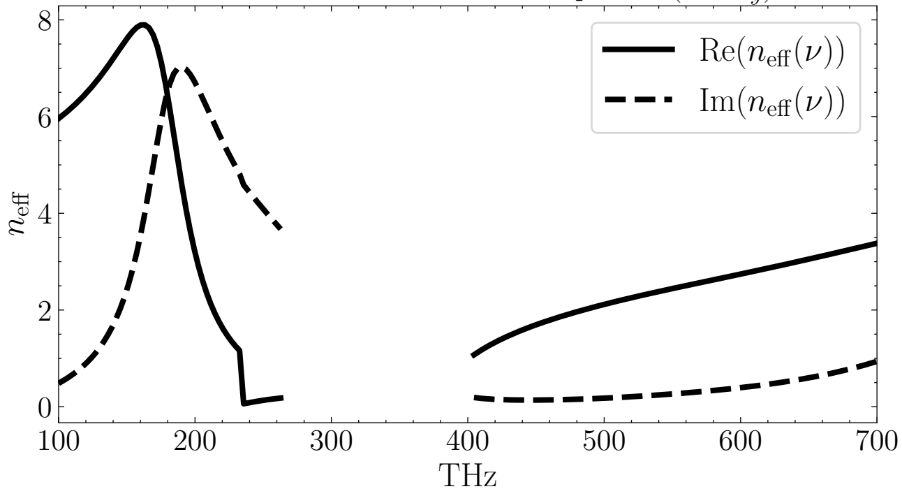
HM-TI surface wave with dissipation ( \mathbf{l} = \mathbf{t}_y )
