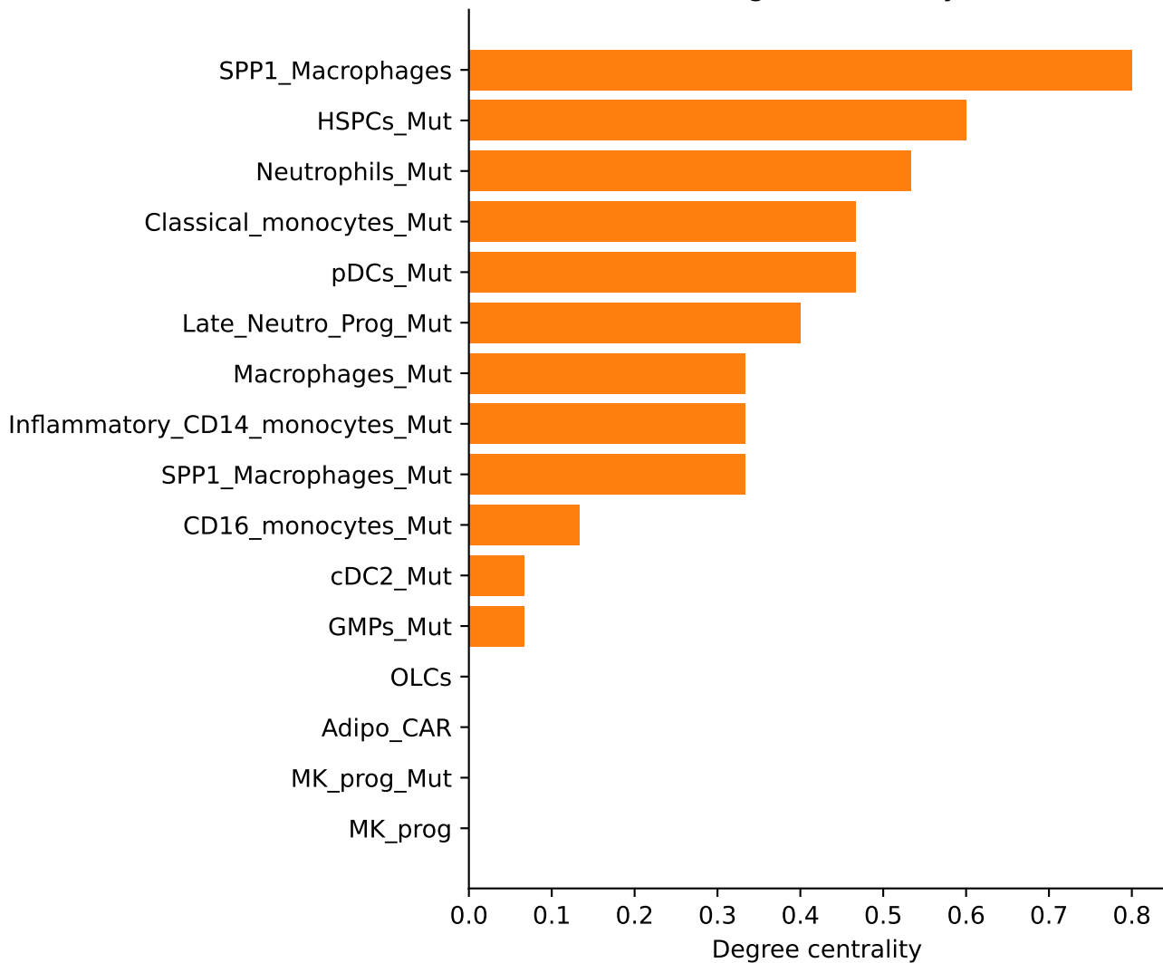
In-degree centrality
