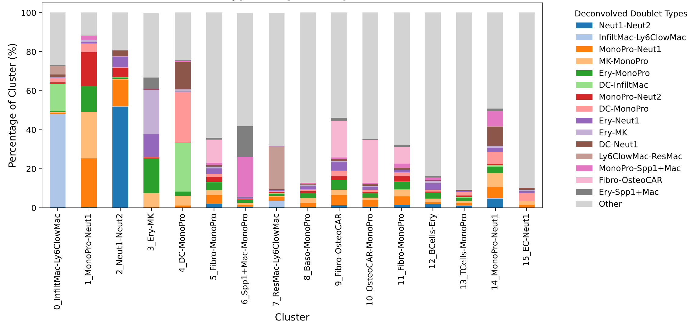
Doublet Type Composition per Cluster
