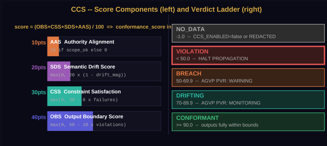
Figure 3. CCS score breakdown (left) and verdict ladder (right). Four components sum to 100 points, normalized to conformance_score in [0.0, 1.0] (BEV-INV-006).
