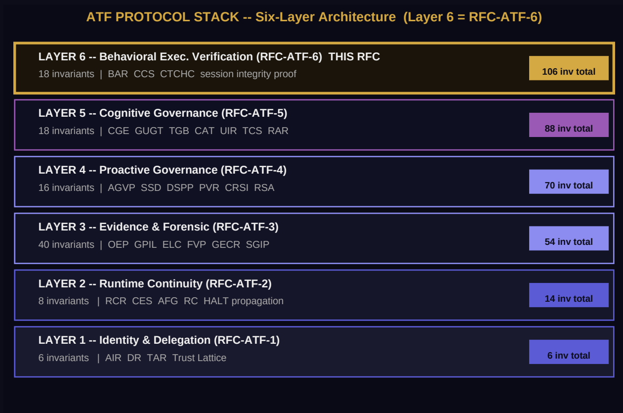
Figure 1. ATF six-layer protocol stack. Layer 6 (gold border) is introduced by RFC-ATF-6.
