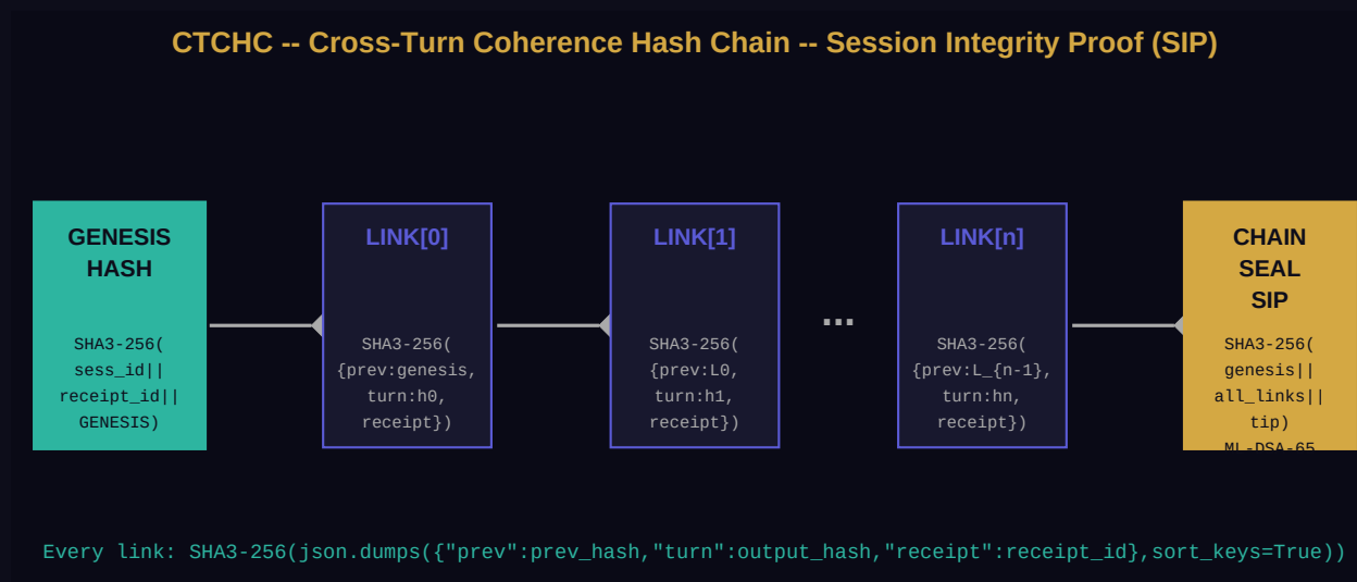
Figure 5. CTCHC hash chain. Genesis hash binds to session_id and governing_receipt_id . Each link encodes prior link, turn output hash, and receipt. ML-DSA-65 chain seal = SIP.
