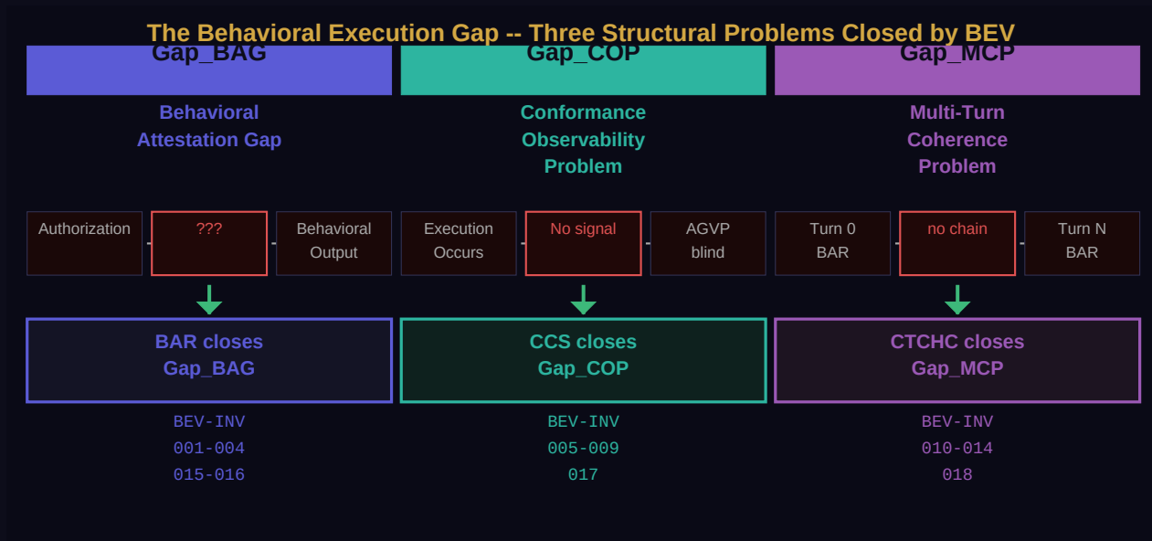
Figure 7. BEV closes the three structural behavioral governance gaps: BAR closes Gap_BAG, CCS closes Gap_COP, and CTCHC closes Gap_MCP.
