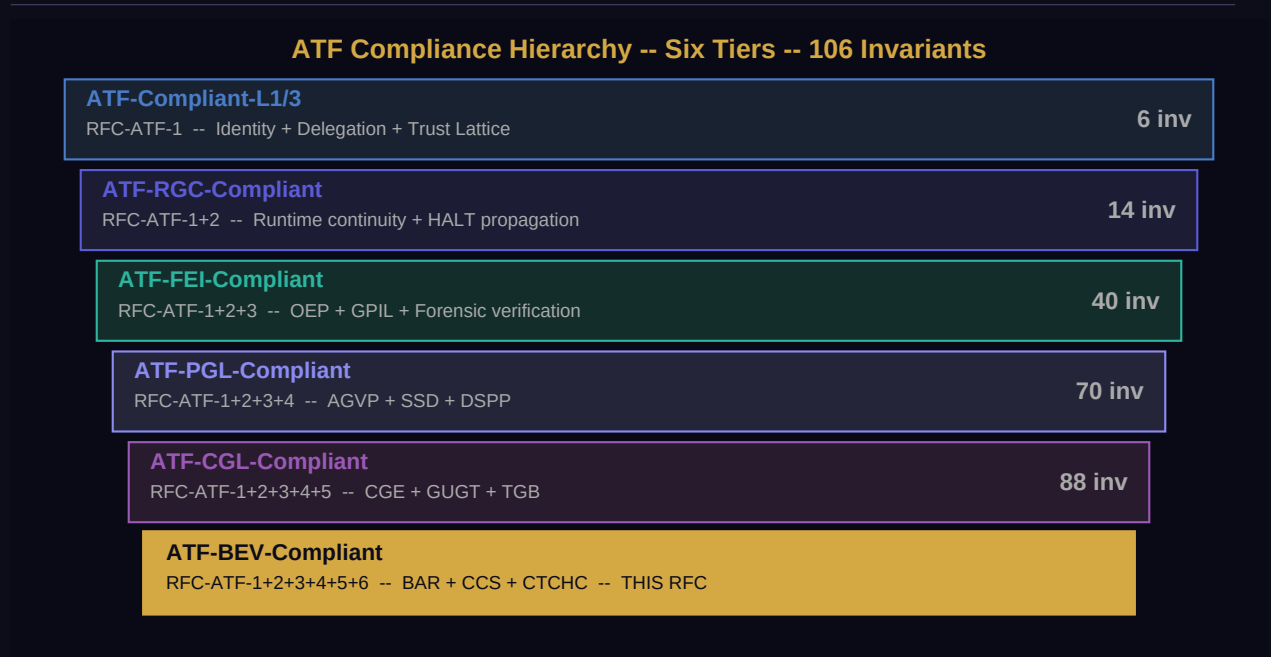
Figure 8. ATF compliance hierarchy. ATF-BEV-Compliant (gold) is the sixth and highest tier.
