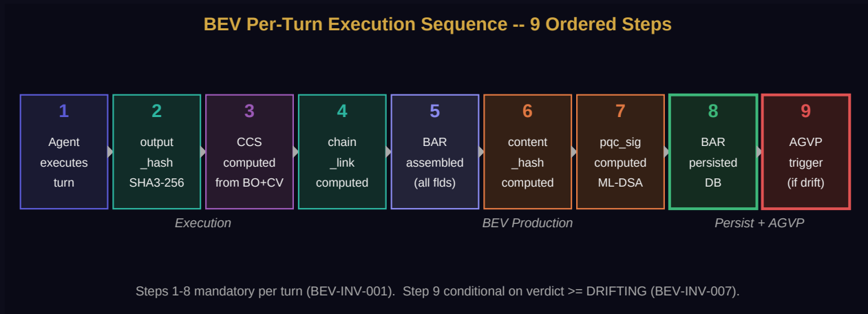
Figure 6. BEV per-turn execution timeline. Steps 1-8 mandatory for every turn (BEV-INV-001). Step 9 conditional on verdict (BEV-INV-007).
