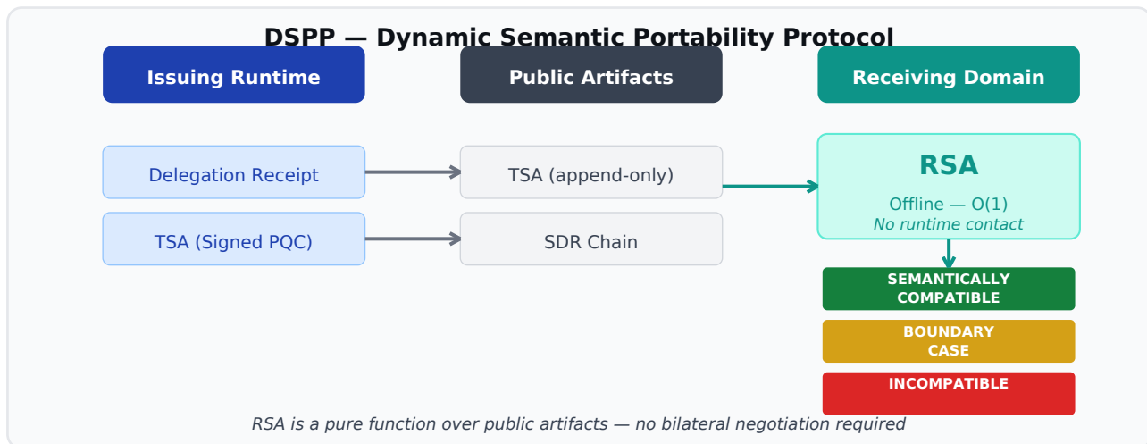
Figure 4 — DSPP: offline RSA computed by any receiving domain without runtime contact
