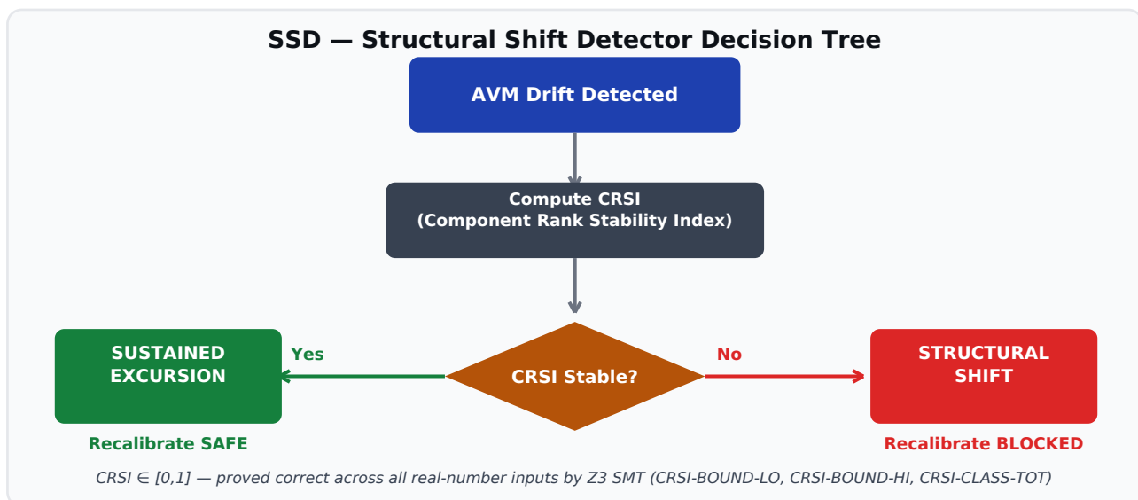
Figure 3 — SSD: CRSI-based classification of drift vs. structural topology shift
