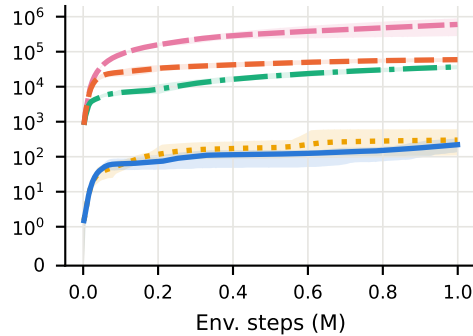
Cumulative hard violations (training, log)
