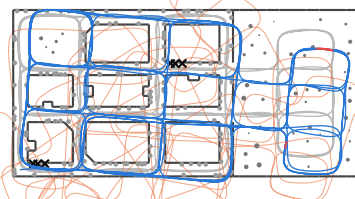
bias1_s5 ATE 14.54 m (aligned 2.87, odo 20.3), 0 wrong
