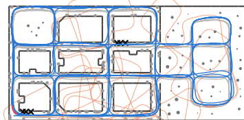
oldsensor_b025 ATE 1.48 m (aligned 0.28, odo 11.0), 0 wrong
