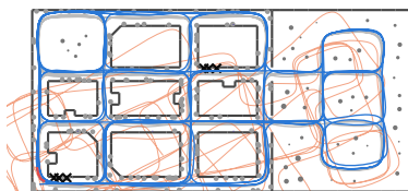
noise5e-6_b025 ATE 0.94 m (aligned 0.28, odo 11.0), 0 wrong
