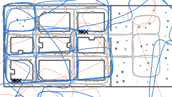
bias2_s4 ATE 19.08 m (aligned 18.17, odo 33.5), 0 wrong
