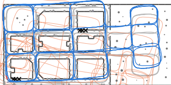
noise1.5e-5_b025 ATE 1.98 m (aligned 1.43, odo 11.0), 1 wrong
