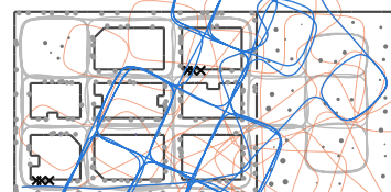
bias1_s5 ATE 14.54 m (aligned 2.87, odo 20.3), 0 wrong
