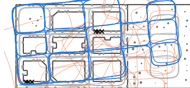
odomnoise_x3_b025 ATE 2.37 m (aligned 0.48, odo 11.7), 0 wrong
