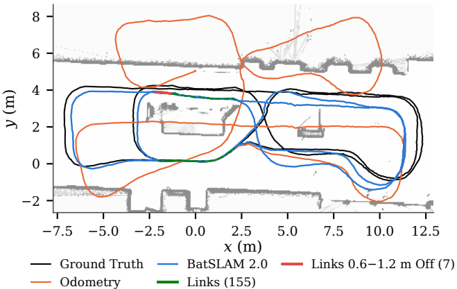
a) One Run: ATE 3.07 m (Odometry) \rightarrow 0.60 m
