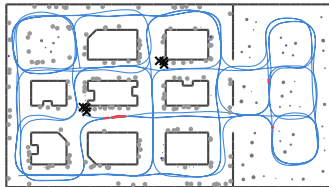
e) BatSLAM 2.0, ATE 0.60 m
