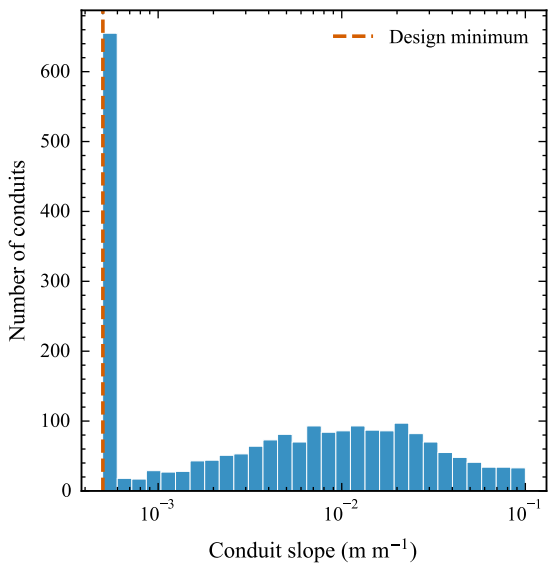
(c) Positive-slope constraint
