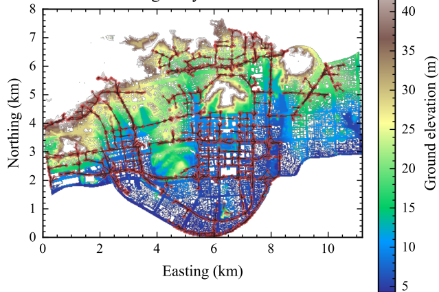
(a) Terrain and gravity-consistent network
