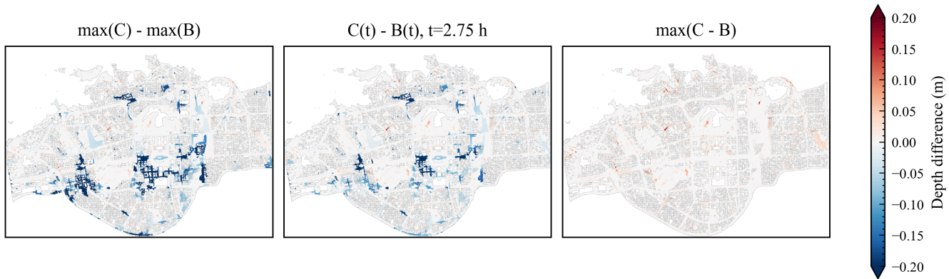
Supplementary Figure S1. Only the middle panel is an instantaneous C-B field. All use fixed +/-0.2 m display limits; extreme values remain in statistics.
