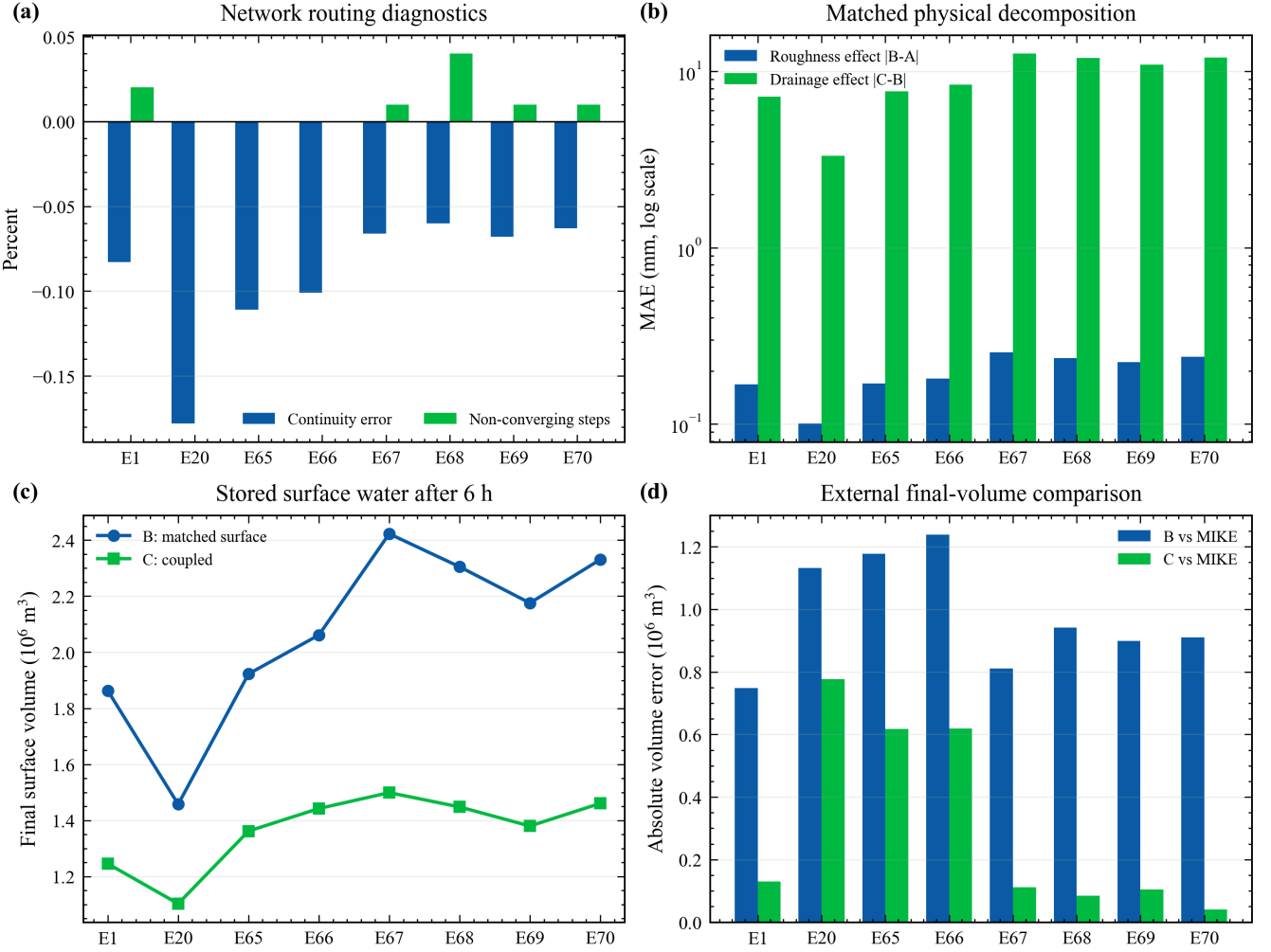
Figure 3. Physical-run quality. Panel (a) reports routing continuity and non-converging steps; the 2% acceptance limits are specified in Section 2.4 rather than drawn on this magnified axis. Panel (b) compares the roughness effect B-A with the sewer effect C-B. Panel (c) shows final surface storage under B and C. Panel (d) gives final-volume discrepancy relative to MIKE. The logarithmic scale in panel (b) is required because the two effects differ by nearly two orders of magnitude.
