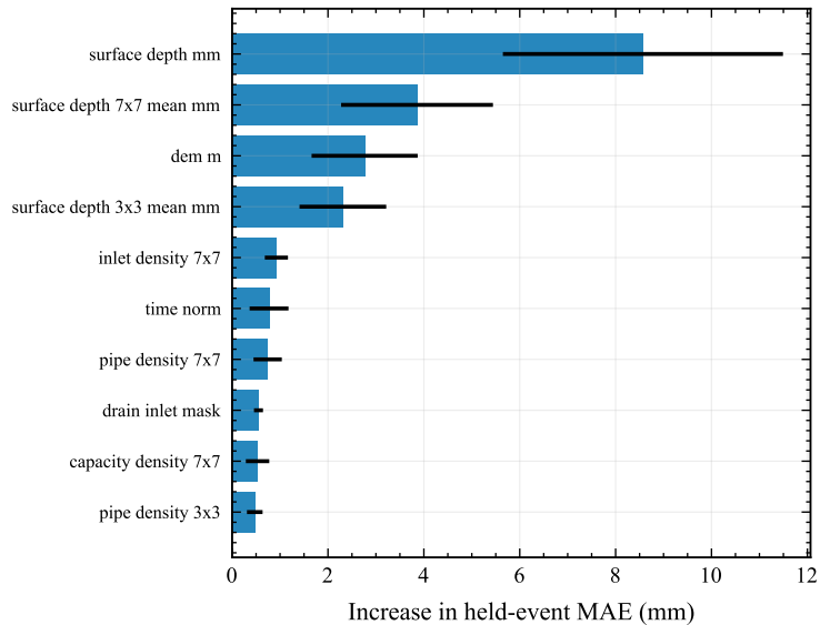
Permutation importance
