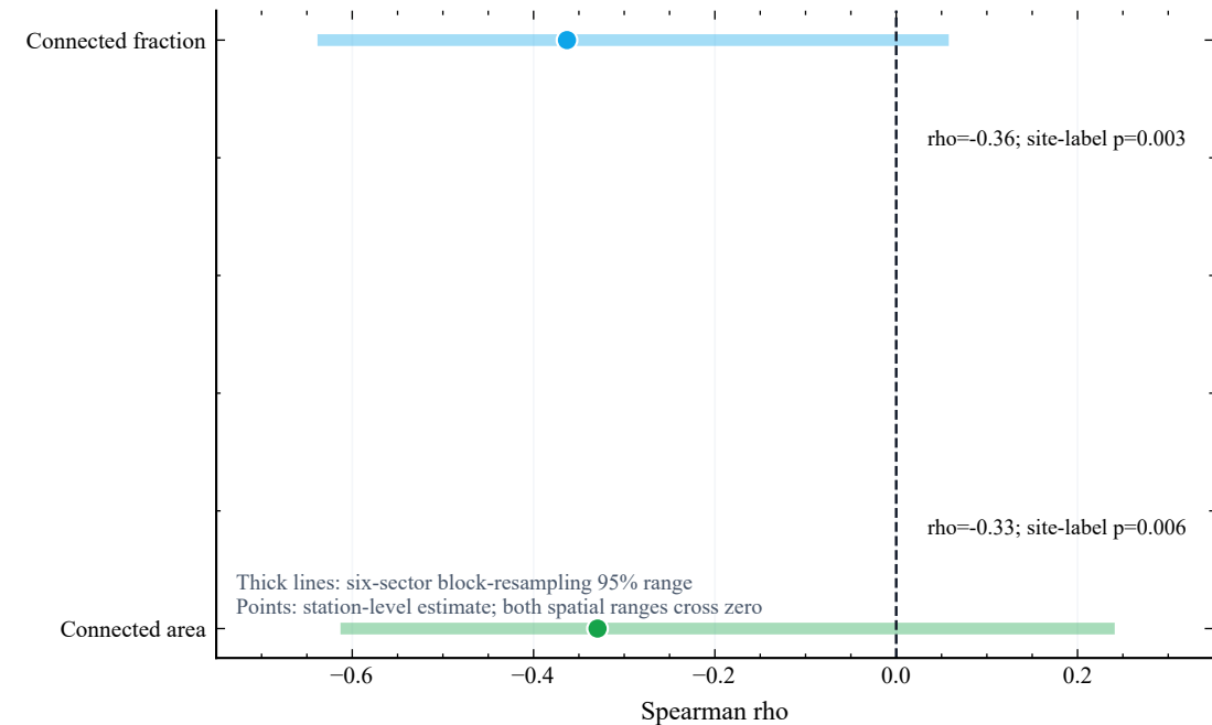
d. Spatial resampling widens the association range
