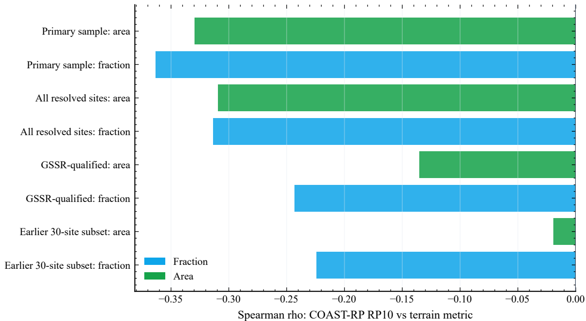
c. Fraction and area metrics give related but not identical rankings
