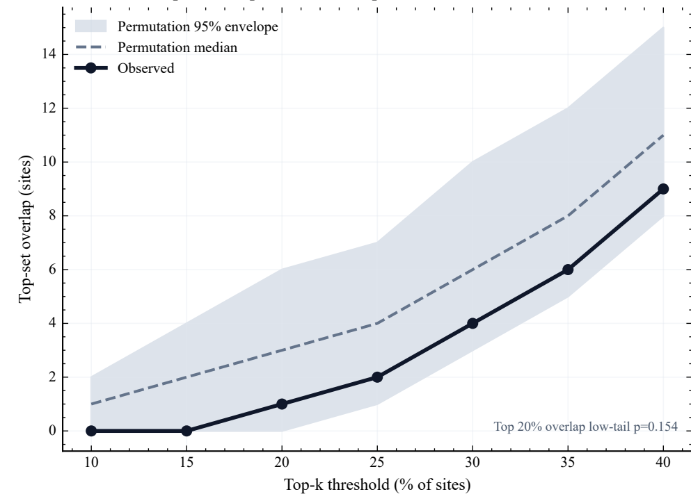
b. Observed top-k overlap relative to the permutation null
