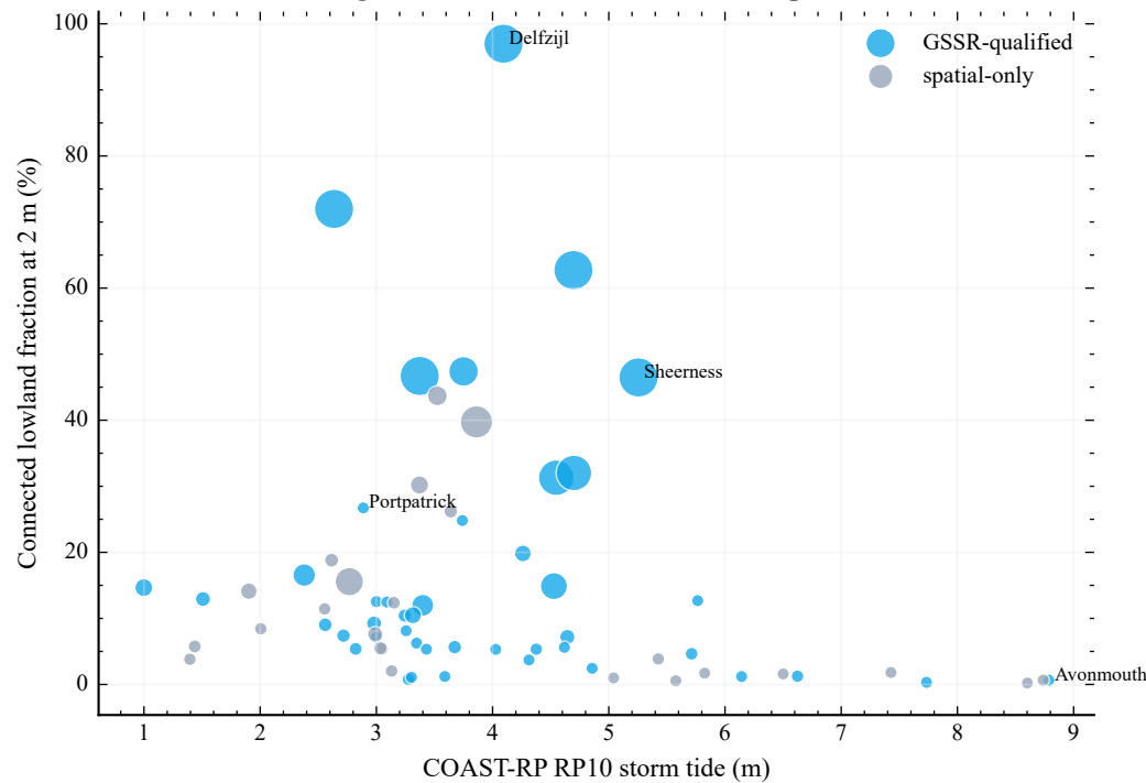
a. Raw storm-tide magnitude versus connected-terrain response
