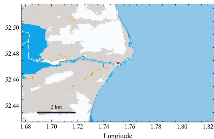
h. Lowestoft RP10 2.38 m; connected 16.6%; area 5.47 km 2
