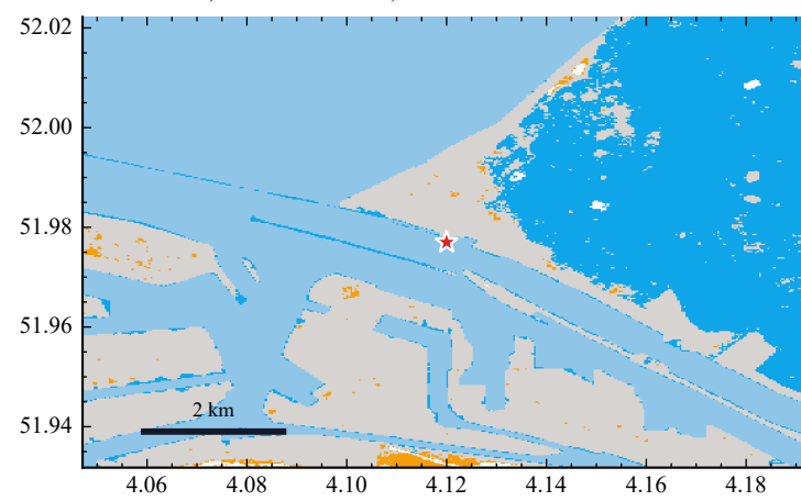
b. Hoek van Holland RP10 3.37 m; connected 46.7%; area 24.96 km 2
