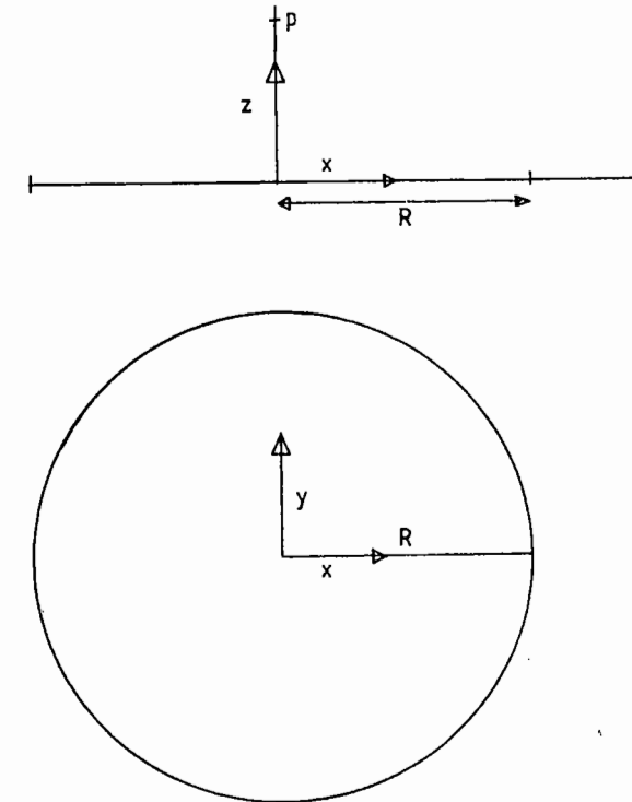
Fig. 4.14. Definition of the source element used in exercise 4.1.
