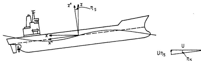
Fig. 3.13. Influence of forward speed U on the body boundary condition for a ship forced to oscillate in pitch \eta_5 .
