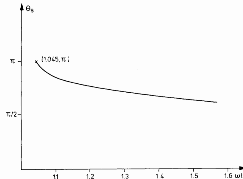
Fig. 7.4. Time development of separation angle \theta_s around a circular cylinder. ( \theta = 0 corresponds to the upstream stagnation point on the cylinder.) The ambient flow velocity is sinusoidal and zero at \omega t = 0 , KC = 3.1 . U_c/U_M = 0 . ( KC and U_c/U_M defined in the beginning of the chapter.)
