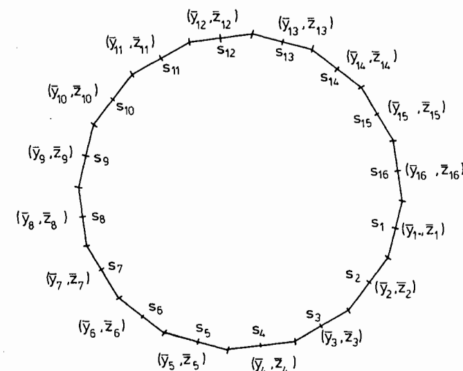
Fig. 4.2. Approximation of a circular cross-section by straight line segments to be used in numerical solutions with the source technique. (\bar{y}_i, \bar{z}_i) = midpoints of segment S_i .
