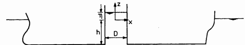
Fig. 3.29. Moonpool dimensions.
