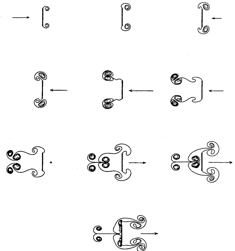
Fig. 7.1. Free shear layer positions at different times for oscillatory crossflow past a flat plate. KC = U_M T/H = \pi ( U_M = velocity amplitude of the ambient flow, T = oscillation period, H = half the height of the plate). U_M t/H = 0.784, 1.584, 1.984, 2.384, 3.184, 3.984, 4.784, 5.584, 6.384, 6.984 (Faltinsen & Pettersen, 1987.)
