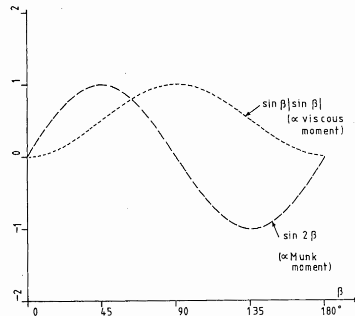
Fig. 6.10. Angular dependence of viscous yaw moment and Munk moment. ( \beta = 0^\circ means current direction towards the stern of the ship.)
