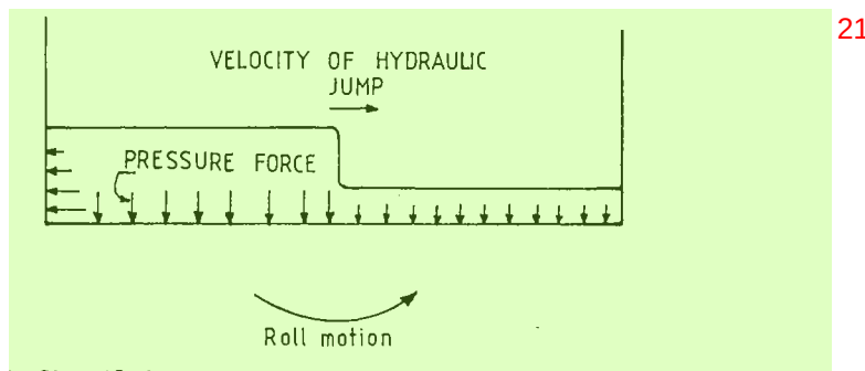
Fig. 3.24. Simplified picture of fluid motion in a shallow water tank at resonance condition shown at the time instant when the roll angle is zero and the roll velocity is maximum.
