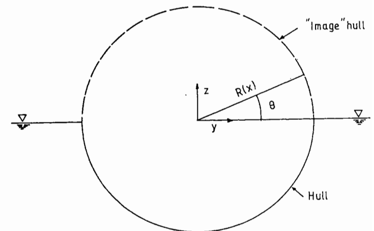
Fig. 6.21. Cross-section of a ship hull and image hull above the free-surface.
