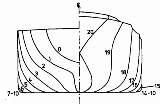
Body plan of tanker model
