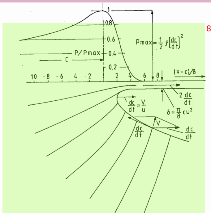
Fig. 9.7. Details of the flow at the intersection between the free surface and a body during impact. ( p = hydrodynamic pressure.) (Wagner, 1932.)
