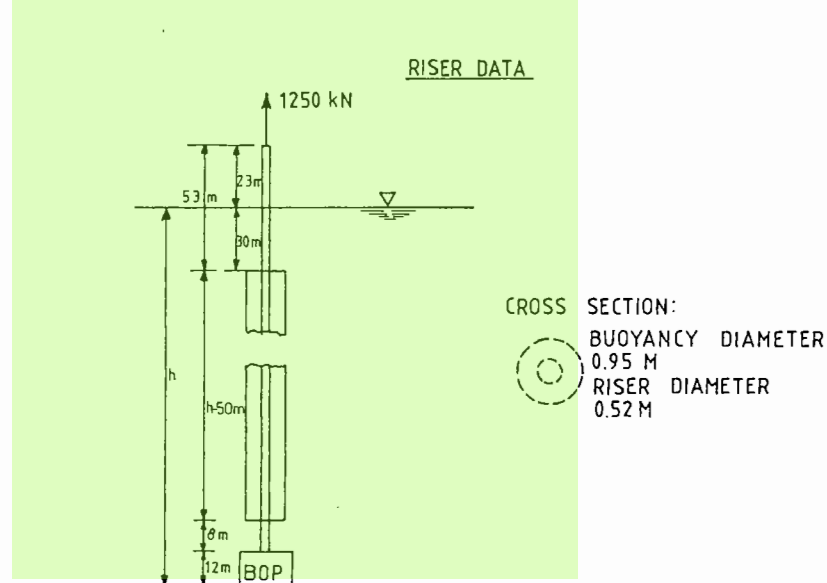
Fig. 6.27. Geometrical particular for riser.
