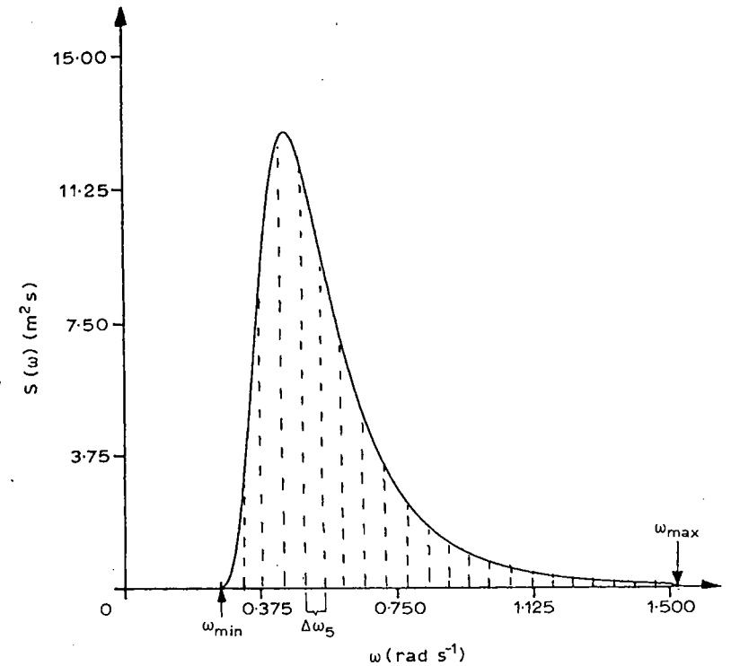
Fig. 5.12. Illustration of how the energy in a wave spectrum S(\omega) can be distributed into energy of regular wave components of circular frequency \omega . (ISSC-spectrum, H_1 = 8 m, T_2 = 10 s, number of wave components N = 22 .) See also Fig. 2.5.
