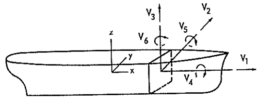
Fig. 9 Sign convention for dynamic wave-load components
